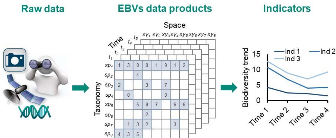
Figure 1. Essential Biodiversity Variables (EBVs) are derived from raw data (i.e., primary observations) obtained, for example, from camera traps, field surveys, satellite remote sensing, and DNA sequencing. Harmonized, standardized and organised as packaged EBV data products , they provide the building blocks for indicator development. EBV data products can be conceptualized as cubes with dimensions of time, space and biology (taxonomy for example). Modified figure from (Kissling et al., 2018a).
