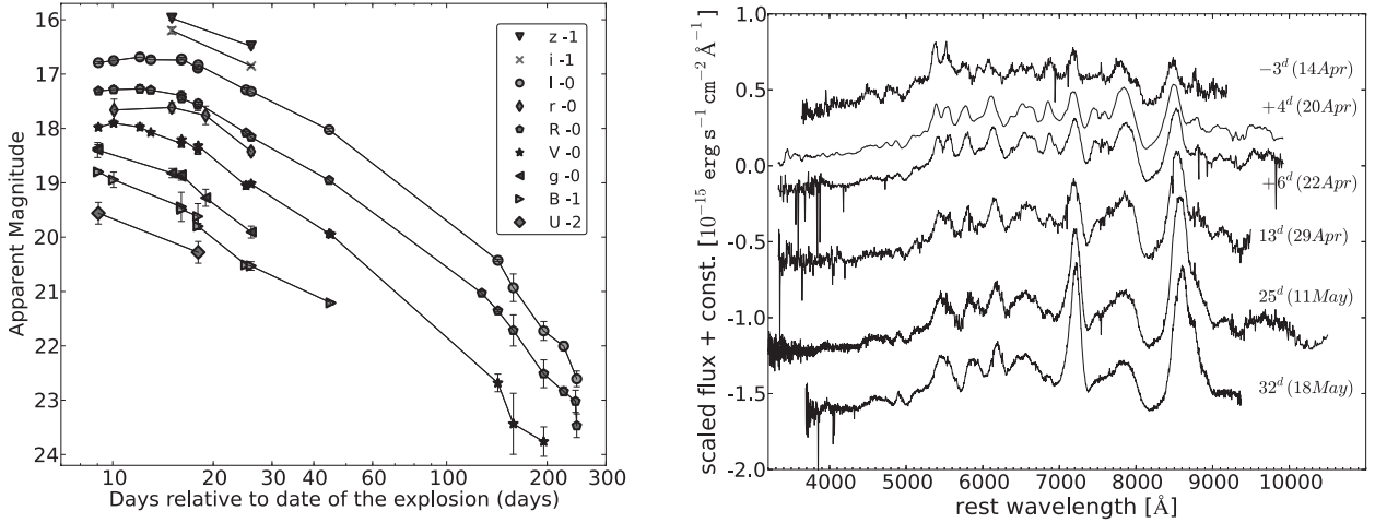
Figure 1. Left: photometry of SN 2012hn in UBgrIz . The date of the explosion has been fixed 12 \pm 3 d before R -band maximum light ( \text{JD}_{\text{exp}} = 245\,6022.5 ). Right: full sequence of photospheric spectra collected for SN 2012hn.
