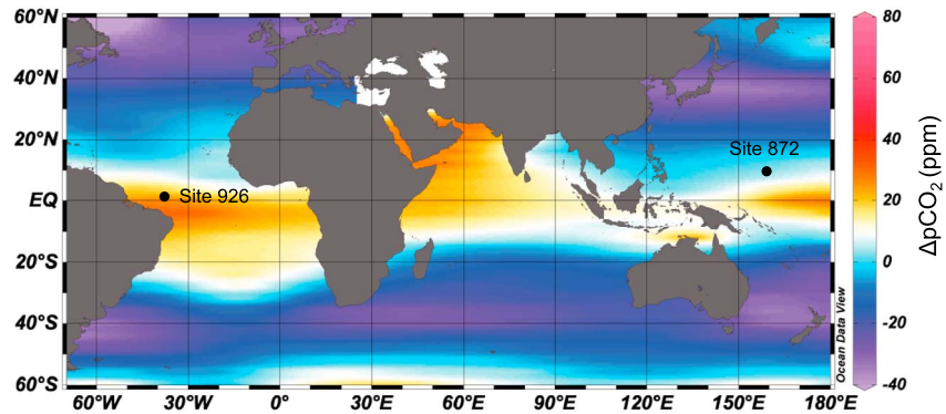
Figure 2. Map of study sites and mean annual air-sea disequilibria with respect to p\text{CO}_2 . The black dots indicate the location of the sites used in this study. Ocean Drilling Program Site 926 ( 3^\circ43.148'N , 42^\circ54.507'W ) is at a water depth of 3,598 m, and the modern extent of disequilibria is approximately +22 ppm. Ocean Drilling Program Site 872C ( 10^\circ05.62'N , 162^\circ52.002'E ) is at a water depth of 1,082 m, and the modern extent of disequilibria is \sim 0 ppm. Data are from Takahashi et al. (2009). Plotted using Ocean Data View (Schlitzer, 2017).
