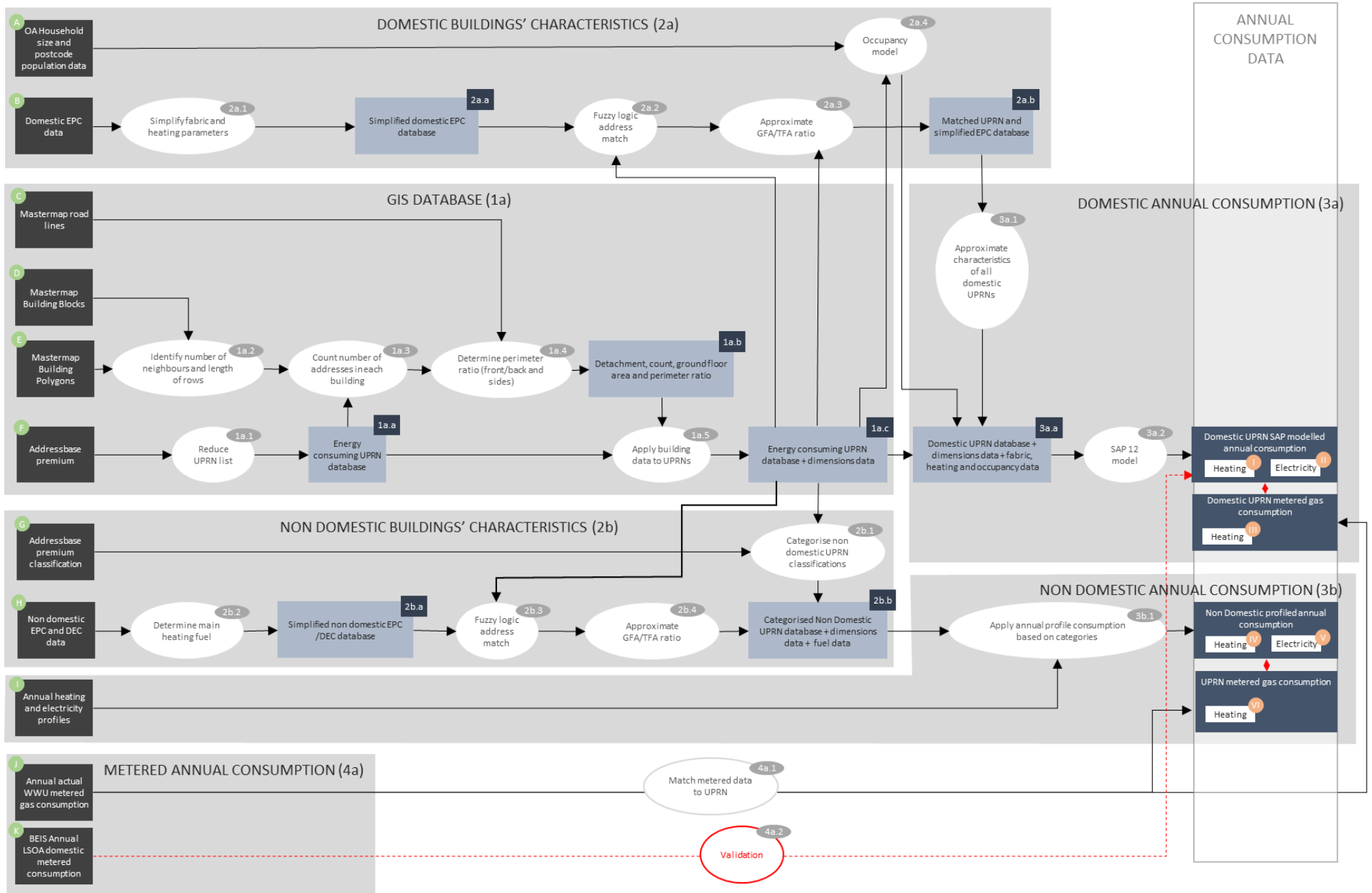
Figure 12: Model structure outline for estimating annual electricity and heating demands per UPRN
