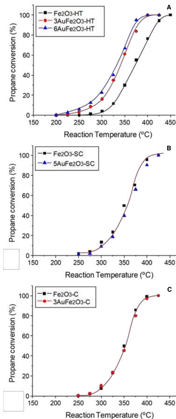
Figure 1. Propane conversion as a function of temperature over gold-free and gold-containing iron oxide catalysts. The supports have been prepared using A) hard template nanocasting method, B) soft chemistry method and C) simple calcination procedure. Reaction conditions: 8,000 vppm propane in air, GHSV = 100,000 h -1 .
