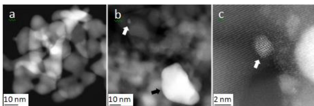
Figure 7. Representative STEM-HAADF micrographs from the 5\text{AuFe}_2\text{O}_3\text{-SC} catalyst. (a) Micrograph showing the typical size and morphology of the iron oxide support grains (b) and (c) small Au nanoparticles about 2 nm in size (indicated by white arrows) as well as relatively large Au particles (black arrow) are clearly evident in the 5\text{AuFe}_2\text{O}_3\text{-SC} catalyst.
