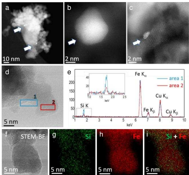
Figure 6. Representative STEM characterization results from the 6\text{AuFe}_2\text{O}_3\text{-HT} catalyst. (a-c) High angle annular dark field (HAADF) Z-contrast micrographs of the catalysts showing Au nanoparticles ranging from 2-6 nm in size (indicated by white arrows). (d) Representative STEM bright field (BF) image of the iron oxide support material in the 6\text{AuFe}_2\text{O}_3\text{-HT} catalyst and (e) the corresponding X-ray energy dispersive spectra (XEDS) acquired from the two regions indicated. The XEDS two spectra in (e) were normalised based on the intensities of the Fe K peaks and Cu K peaks (the latter of which originates from the TEM grid). (f) STEM-BF image and the corresponding XEDS maps of (g) Si and (h) Fe. (i) shows an overlay of the Si (green) and Fe (red) map.
