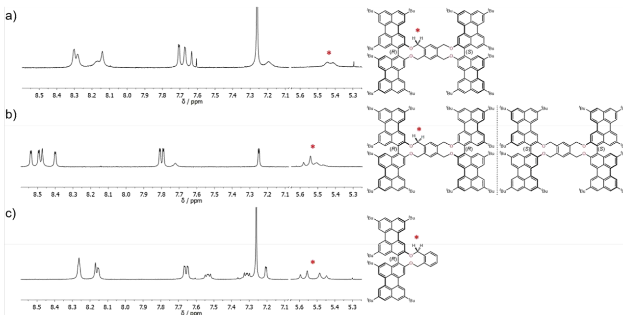
Figure 3. 300 MHz ^1\text{H-NMR} spectrum of molecules a) meso - 3 c in \text{CDCl}_3 at 45 °C, b) ( R,S )- 3 c in (\text{CD}_3)_2\text{CO} at r.t., and c) ( R,R )- 3 d in \text{CDCl}_3 at r.t.
