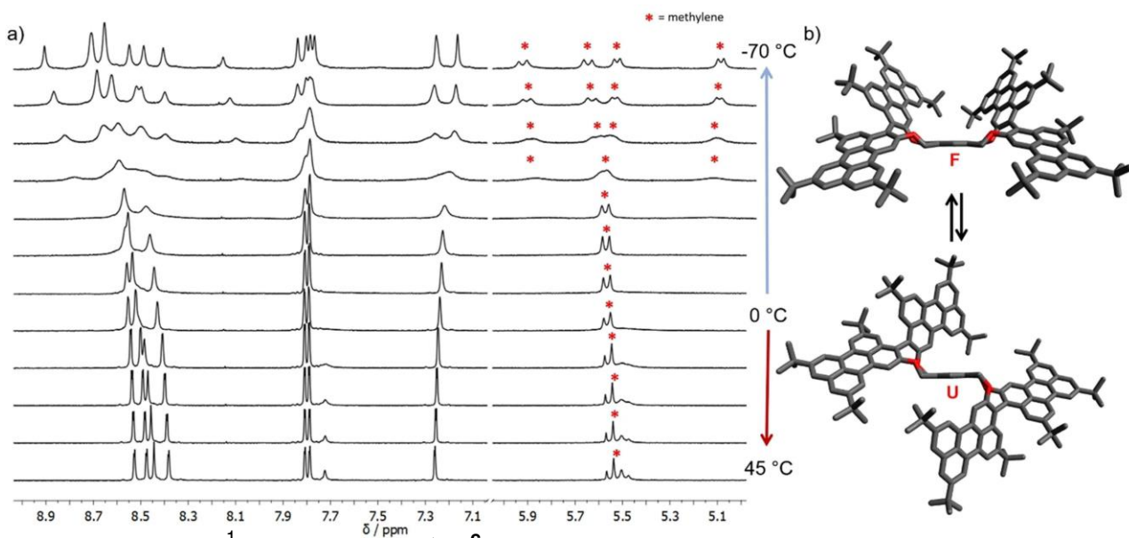
Figure 4. a) 400 MHz VT ^1\text{H-NMR} spectra of ( R,S )- 3 c at 45, 35, 25, 15, 0, 10, 20, 30, 40, 50, 60, 70 °C (bottom to top) in (\text{D}_6) acetone, and b) schematic representation of the conformational inversion process between the folded (F) and unfolded (U) conformers (hydrogens are omitted for clarity).
