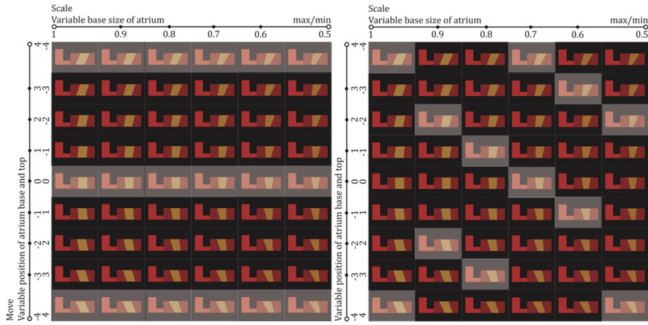
Fig. 4. Training data set A and B (left to right): The matrix represents the solution space of 54 design variants. The simulations from which the training data was extracted have been highlighted. Training data set A comprised 18 simulations – 3 from every column of the matrix. For training data set B, 2 simulations were selected from every column of the matrix.
