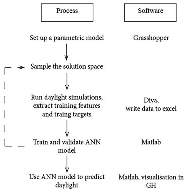
Fig. 2. ANN-integrated workflow
