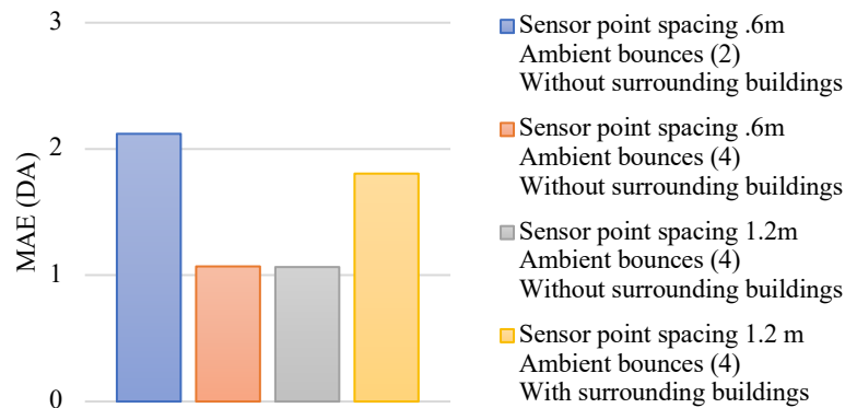
Fig. 6. ANN sensitivities to simulation settings
