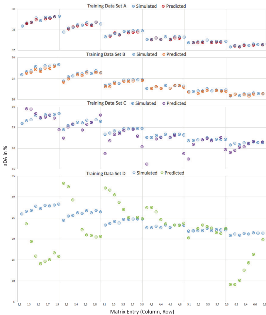
Fig. 8. sDA performance of the 54 generated design solutions: Predicted and simulated sDA for training data sets A to D
