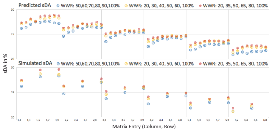
Fig. 9. Predicted and simulated sDA performance for WWR distributions
