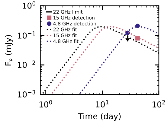
Figure 16. The best-fitting SSA model (dotted lines) plotted over the observations (symbols) at 22 GHz (black), 15 GHz (pink), and 4.8 GHz (indigo). These data are best fit by a shock velocity of \sim 1.4 \times 10^4 km s ^{-1} and a density of K = 4.51 \times 10^{11} g cm ^{-3} .
