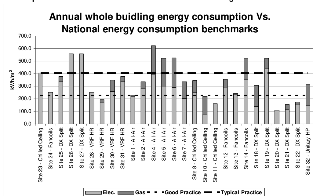
Figure 1: Comparison of annual whole building energy consumption to national energy consumption benchmarks for air conditioned office buildings.
