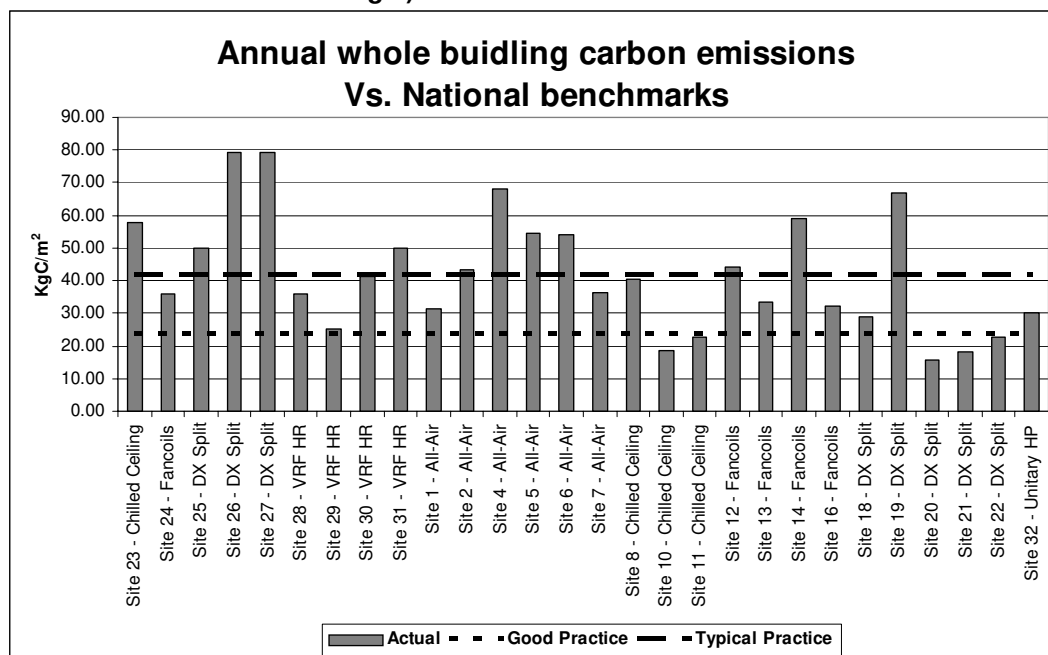
Figure 2: Comparison of annual whole building carbon emissions to national benchmarks for air conditioned office buildings.)
