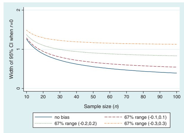
Figure 4 Effect of ranges for an additive bias on the width of the 95% CI for the bias-adjusted correlation coefficient
