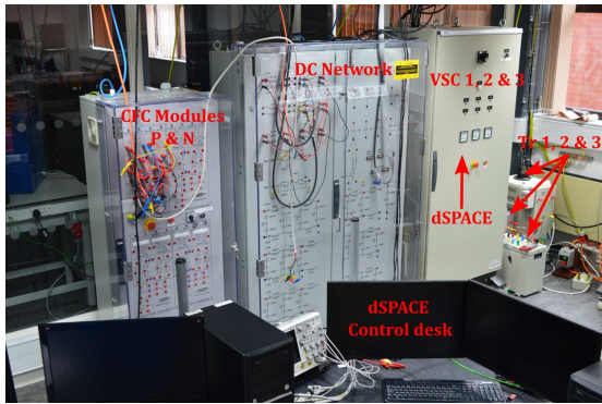
Fig. 12. Experimental setup.
