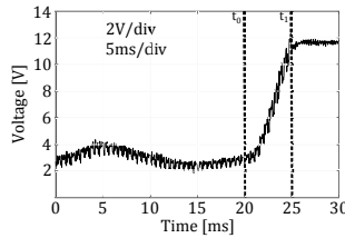
Fig. 24. 1B-CFC capacitor voltage during a pole-to-pole dc fault (experimental results).
