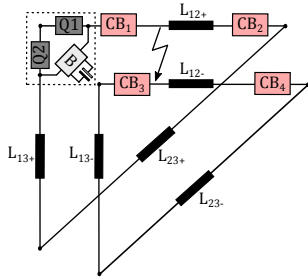
Fig. 22. Pole-to-pole fault location.
