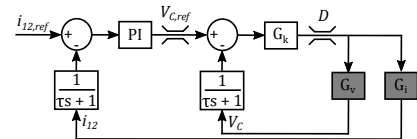
Fig. 6. 1B-CFC controller.
