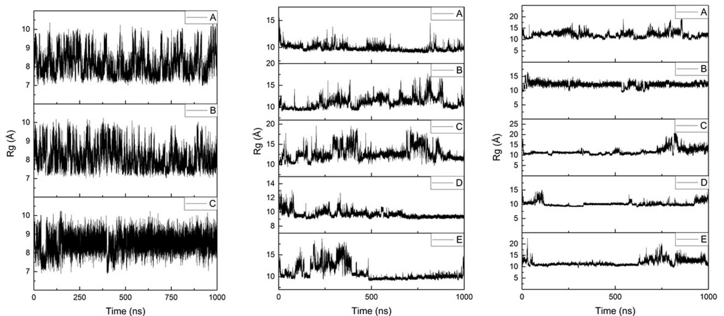
Fig 3. Rg plots for Al-A \beta 16, Al-A \beta 40 and Al-A \beta 42 simulations.
