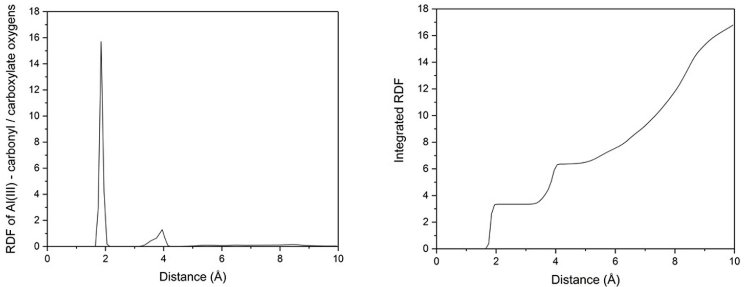
Fig 2. (a) RDF and (b) integrated RDF of Al-oxygen distances in Al-A \beta 42.
