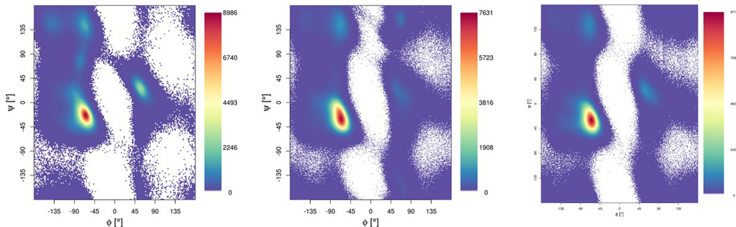
Fig 5. Ramachandran plots for simulations of Al-A \beta 16, Al-A \beta 40 and Al-A \beta 42.
