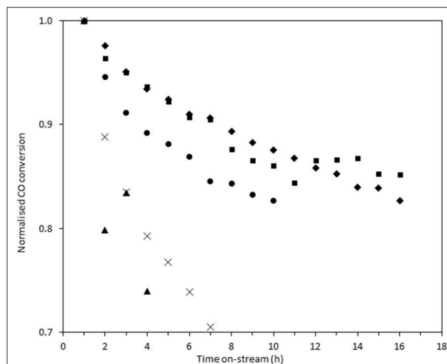
FIGURE 8 | Normalized on-stream conversion of Au/Ce 0.2 Ti 0.8 O 2 (■), Au/Ce 0.5 Ti 0.5 O 2 (◆), Au/Ce 0.5 Zr 0.5 O 2 (●), Au/Ce 0.9 Ti 0.1 O 2 (×), and Au/CeO 2 (▲) in LTS reaction 0.150 g catalyst, 150°C, 100 ml min -1 , 2% CO, 2% CO 2 , 7.5% H 2 O, 8.1% H 2 , 80.4% N 2 . Conversions were normalized against their conversion at 1 h on-stream.
