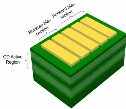
Figure 1: Schematic of the segmented contact method for a monolithic integrated QD laser and QD modulator for short and medium reach optical interconnects capable of operating up to 398 K.
