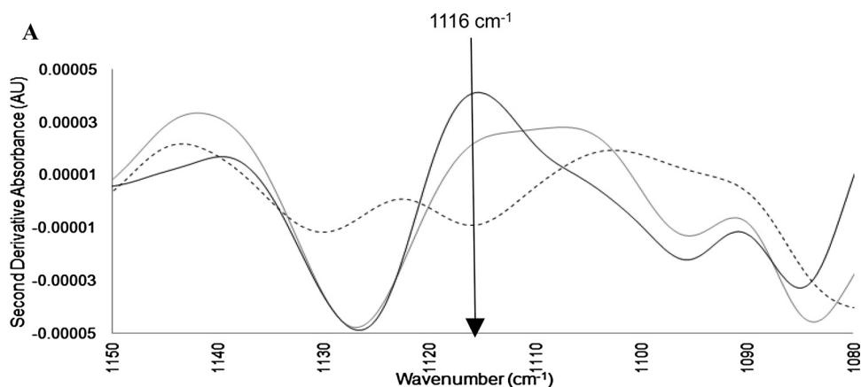
Fig. 3. Mean second derivative spectra for OligoG CF-5/20 treated and untreated sputum surrounding 1116 cm -1 indicating IR absorbance from sulphated-Lewis x antigen. (a) The IR peak at 1116 cm -1 was lost following OligoG CF-5/20 incubation. The new peak occurring at 1096 cm -1 in the treated spectrum is suggestive of interaction between OligoG CF-5/20 and sulphated- sulphated-Lewis x antigen. (b) Boxplots of second derivative negative peak height distributions centered around 1116 cm -1 in untreated and treated samples respectively. Treated sputum, solid grey line; untreated sputum, black dashed line; OligoG CF-5/20, light-grey dashed line. * P < 0.008, mean of n = 3 replicates.
