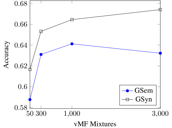
Figure 1: Accuracy vs number of vMF mixtures on the Google word analogy dataset for our model.
