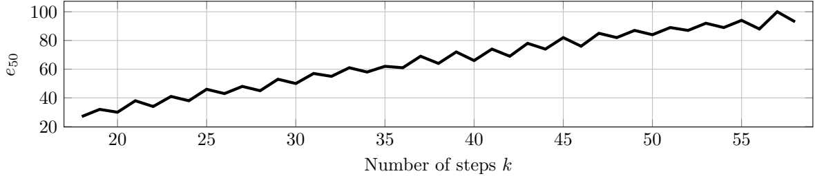
(c) The number e_{50} of not-equals constraints at phase transition.
