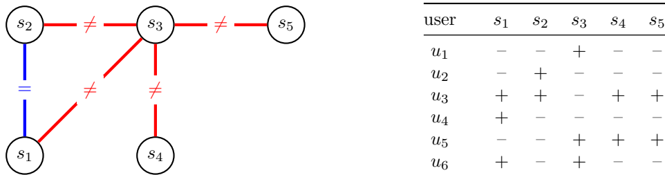
Figure 1: An example of a WSP instance with k = 5 and n = 6 . On the left, each step is represented with a node, and each constraint with an edge (in general, a constraint is represented with a hyper-edge but in this example all the constraints have scopes of size two). Red edges (marked with “ \neq ”) represent not-equals constraints, and blue edges (marked with “ = ”) represent equals constraints. The table on the right gives authorisations A(u) , where ‘+’ means authorised and ‘-’ means unauthorised.
