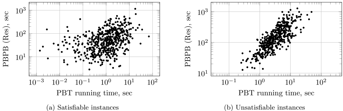
Figure 11: Correlation between PBT and PBPB (Res) running times on instances of size k = 40 . 1000 instances used in this experiment (about 500 satisfiable and 500 unsatisfiable).
