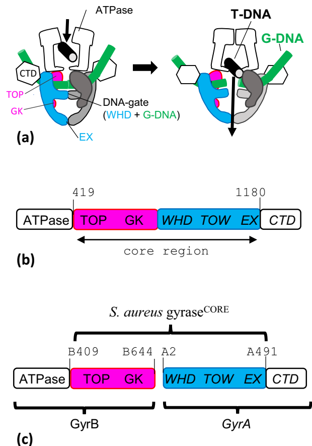
Fig. 1. Schematic of type IIA topoisomerases. (A) Simplified schematic of the action of type IIA topoisomerases, such as yeast topoisomerase II (topo II), DNA gyrase and topoisomerase IV. A segment of DNA (T-DNA) is transported by capture through the ATPase domains interface and passes through a transient double-strand break established in the G-DNA (forming a DNA “gate” interface with the WHD domain). The DNA then exits the enzyme through the exit gate (EX). (B) Eukaryotic topo IIs are homodimers, and many key structures have been determined with a “core” region (419–1180) encompassing the TOPRIM domain (TOP), the Greek key fold, the winged-helix domain (WHD), the Tower (TOW) and the exit gate (EX). (C) Fusing the C-terminal region of S. aureus GyrB (residue 409 to 644) to the N-terminal region of GyrA (residue 2 to 491) gives an “equivalent” construct. The Greek key can be deleted from this core construct in S. aureus gyrase.
