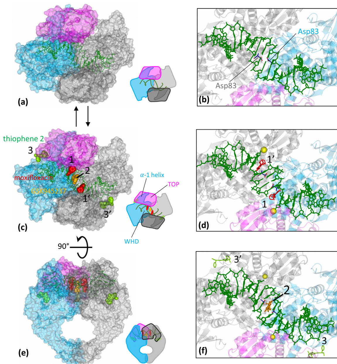
Fig. 3. Inhibitors (I) can stabilize the cleaved state through binding at different positions. (A) View of the un-cleaved binary complex equivalent to Fig. 2c. (B) Closer view of the binary complex (6FQV) showing the proximity of the two Asp83 residues at the WHDs interface. (C) Global view of compound binding sites on the S. aureus gyrase CORE illustrated by moxifloxacin (in sites 1 and 1'), GSK299423 (in site 2) and thiophene 2 (in sites 3 and 3'). The structure represented is a composite between a thiophene 2 and GSK945237 bound structure (PDB code: 5NPP) and a moxifloxacin-bound structure (PDB code: 5CDQ). (D) Closer view of the moxifloxacin structure (5CDQ) showing moxifloxacin (I1 and I201), Mn 2+ (yellow sphere) and the separation of the Asp83 residues. (E) Alternative view of the composite representation shown in panel C. (F) Closer view of the NBTIs/thiophene structure (5NPP) showing GSK945237 (2), and thiophene 2 (3 and 3'), Mn 2+ (yellow sphere) and the separation of the two Asp83 residues.
