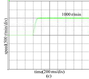
Fig.9. Startup experiment contrast under different control strategies. (a) Experimental results under PI controller. (b) Experimental results under SMSC using the reaching law in reference [8] (RLR8). (c) Experimental results under SMSC using NSMRL.
