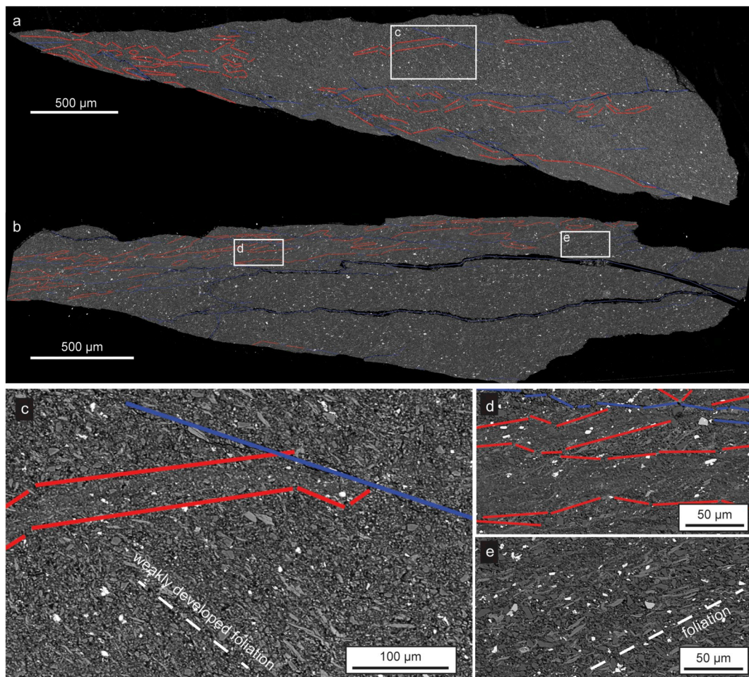
Fig. 11. Overview microstructures of the felsic samples deformed at a constant velocity of 1 \mu\text{m/s} for 5 mm at an effective normal stress of 100 MPa and at (a) room temperature and (b) 500 ^{\circ}\text{C} . Cracks are indicated by blue lines, zones of grain size reduction are indicated by red lines. Sample thickness in both cases is about 800 \mu\text{m} and shear sense is top-to-the right. White boxes indicate the location of the close-ups shown in (c) for the relation between cracks, zones of finer grain size, and poorly developed foliation in the room temperature sample, and in (d) and (e) for the 500 ^{\circ}\text{C} sample. (For interpretation of the references to colour in this figure legend, the reader is referred to the web version of this article.)
