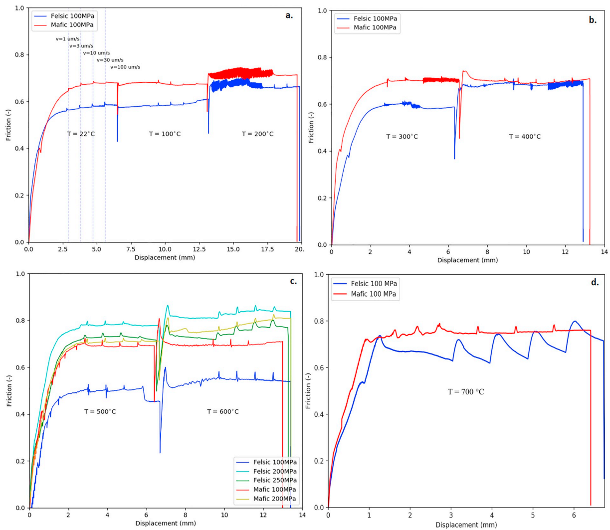
Fig. 3. Plots of the evolution of friction with displacement. Temperature and effective normal stress as indicated. Sliding velocity was stepped through the range 1-3-10-30-100 with a displacement for each individual step of 3-0.9-0.9-0.9-0.9 mm, respectively.
