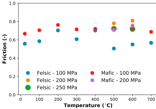
Fig. 4. Apparent coefficient of friction (=shear stress/effective normal stress, ignoring cohesion) at the end of the step at 1 \mu\text{m/s} as a function of temperature. Measurement errors are smaller than the symbol size, reproducibility was not tested.
