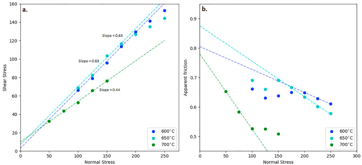
Fig. 9. a) Plot of shear stress as a function of effective normal stress with linear fits to the data for temperatures of 600, 650 and 700 °C. b) Plot of apparent friction as a function of effective normal stress for temperatures of 600, 650 and 700 °C.
