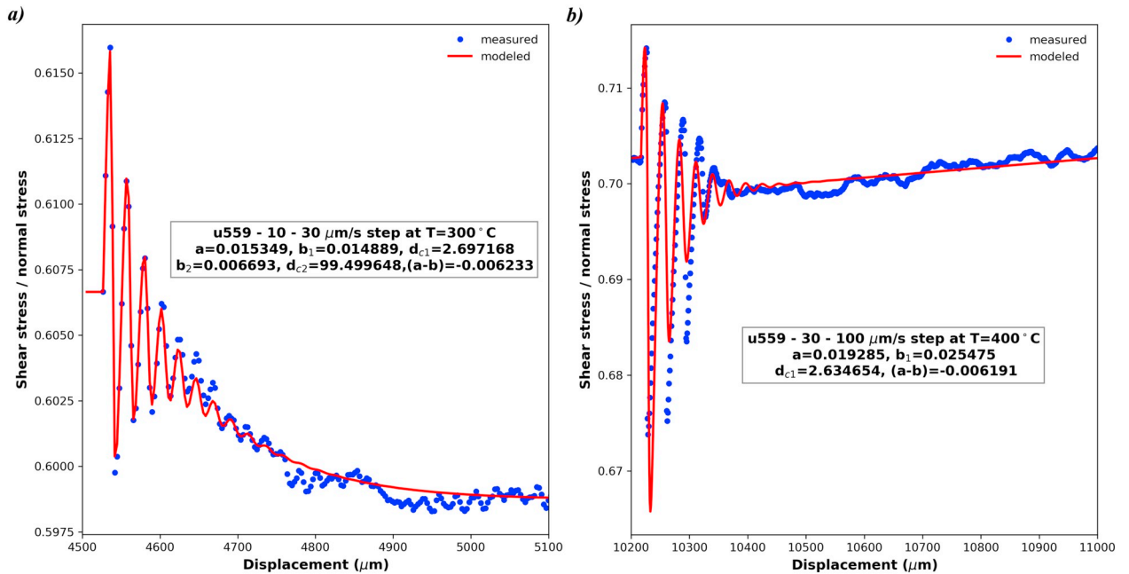
Fig. 5. Examples of model fits to the experimental data from experiment u559, which was done on the felsic sample M01 at temperatures of 300 and 400 °C. The largest standard deviations of the misfits to the models are always on the critical displacement(s) and can be up to 30%, as in the case of the example shown in a), whereas standard deviations on the values of a , b_1 and b_2 are generally < 1\% .
