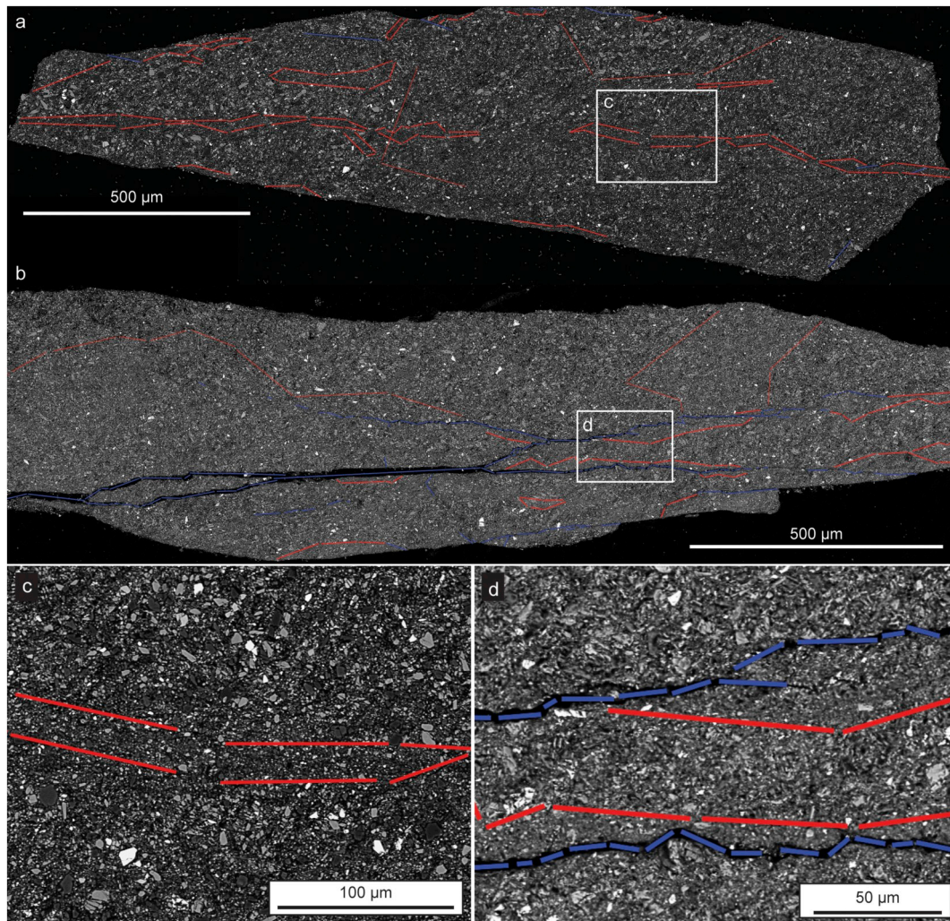
Fig. 10. Overview microstructures of the mafic samples deformed at a constant velocity of 1 \mu\text{m/s} for 5 mm at an effective normal stress of 100 MPa and at (a) room temperature and (b) 500 ^{\circ}\text{C} . Cracks are indicated by blue lines, zones of grain size reduction are indicated by red lines. Sample thickness in both cases is about 800 \mu\text{m} and shear sense is top-to-the-right. (For interpretation of the references to colour in this figure legend, the reader is referred to the web version of this article.)
