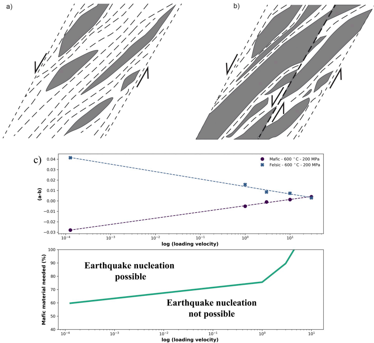
Fig. 15. Schematic of the envisioned fault zone structure at depth, with transposed and dismembered layers of mafic/velocity-weakening material (grey) within a felsic/velocity-strengthening matrix (white with dashed lines denoting foliation). The mafic layers are inferred to have been transposed within a ductile shear zone; the timing of transposition and the original orientation of the layers is not inferred nor implied.
