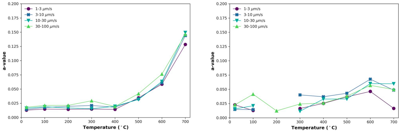
Fig. 8. a) Plot of the value of a , the direct effect parameter in rate-and-state friction as a function of temperature for the felsic sample. b) Plot of the value of a , the direct effect parameter in rate-and-state friction as a function of temperature for the mafic sample.
