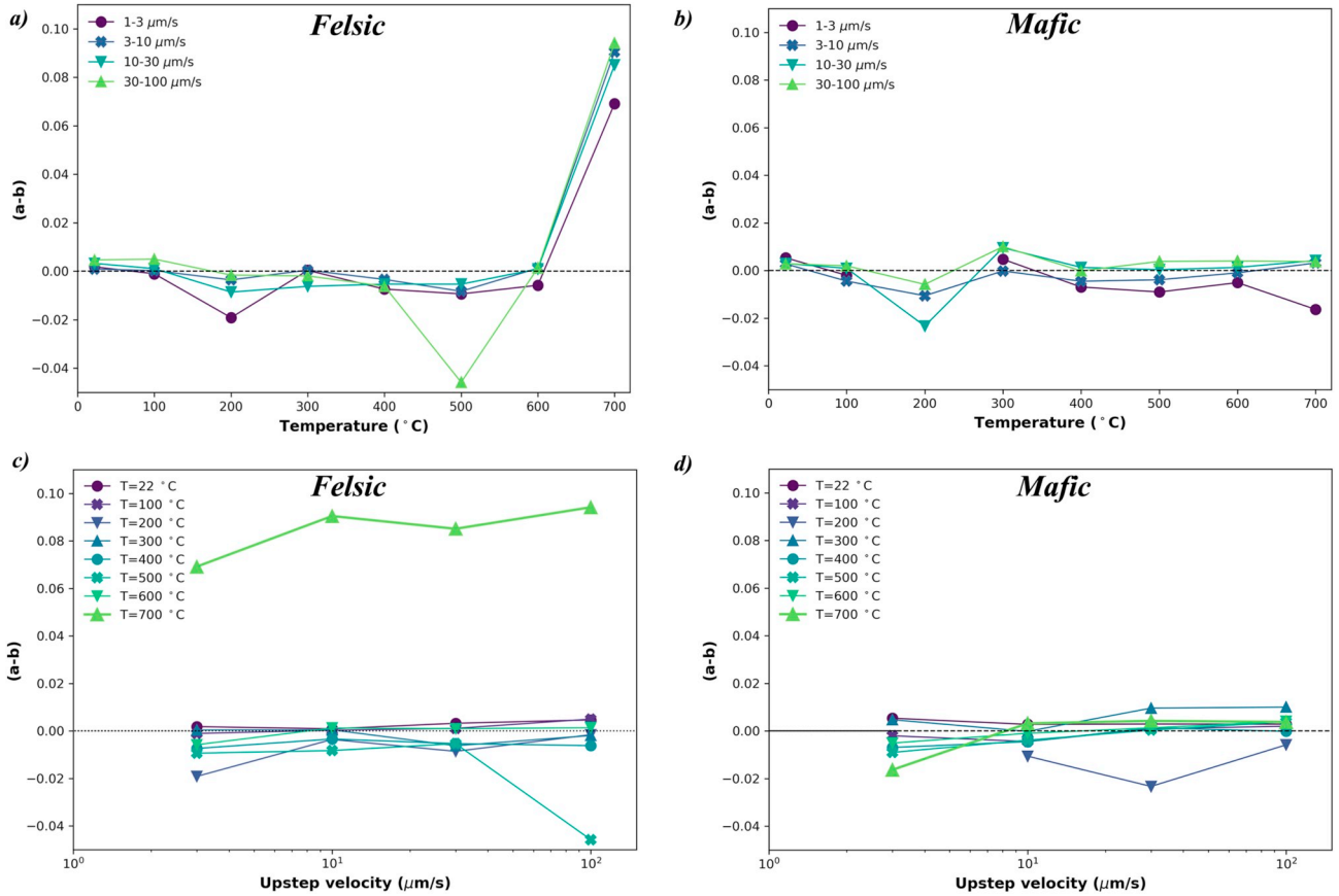
Fig. 6. Plots of (a-b) as a function of temperature (a,b) as well as sliding velocity (c,d) for all experiments performed at 100 MPa effective normal stress (see Tables 2–4).
