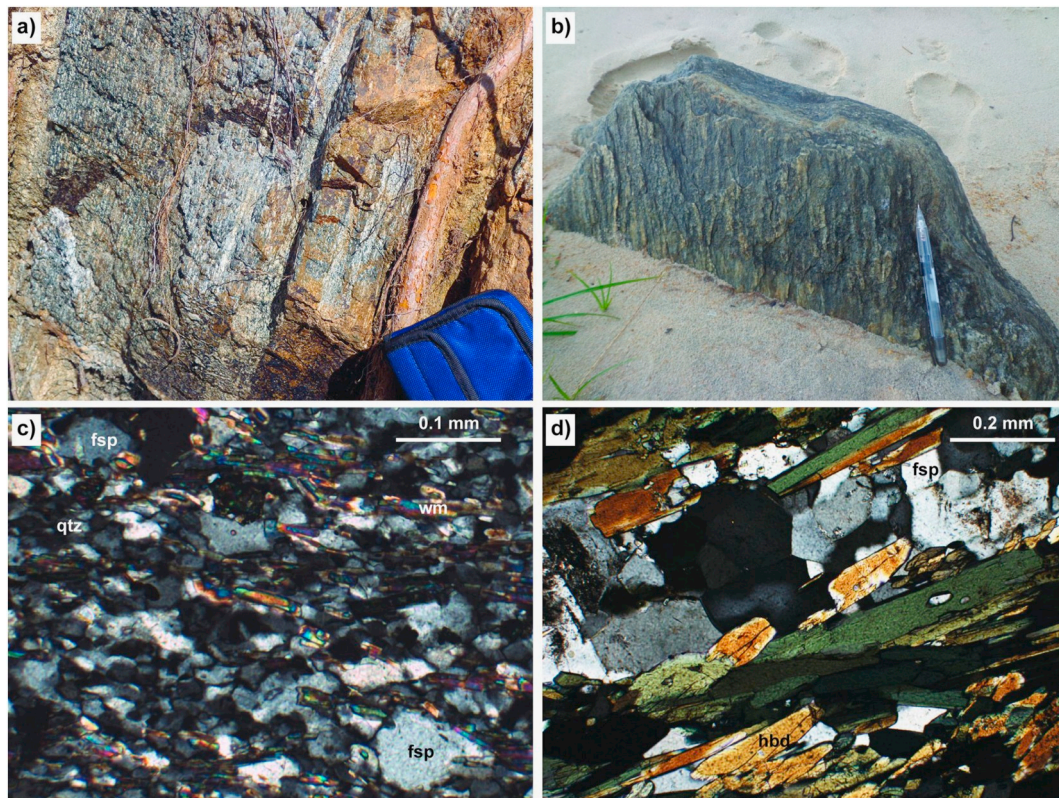
Fig. 2. a) Photo of the outcrop from which sample M01 (felsic) was obtained. See text for description. Compass for scale is \sim 15 \times 15 cm. b) Photo of the outcrop from which sample M17 (mafic) was obtained. See text for description. Pen for scale is 15 cm long. c) Micrograph of a thin section from the hand specimen from which sample M01 was obtained. d) Micrograph of a thin section from the hand specimen from which sample M17 was obtained.
