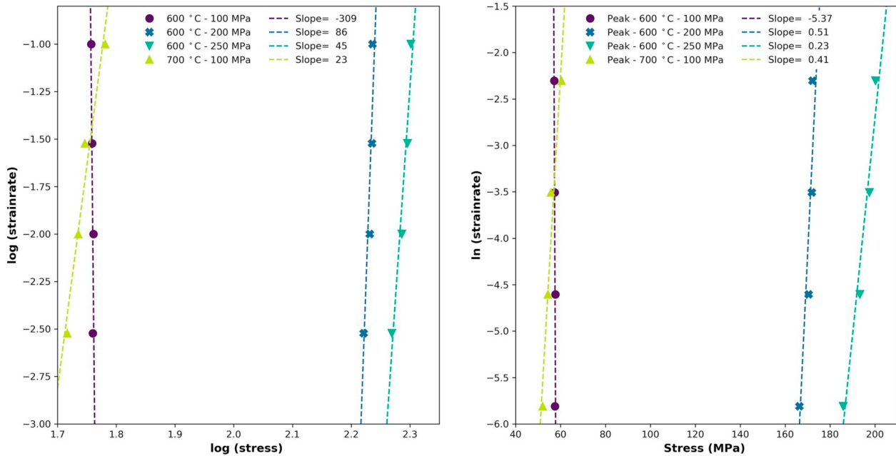
Fig. 14. Plots of the peak shear stress for the three different up-step velocities (3-10-30 \mu\text{m/s} ) which have been converted to strain rates by dividing over the gouge layer thickness of 1 mm. a) Plot in log-log space, showing the stress exponent in a power flow law as the slope b) Plot in semi-log space, showing the pre-exponent constant in an exponential flow law as the slope.
