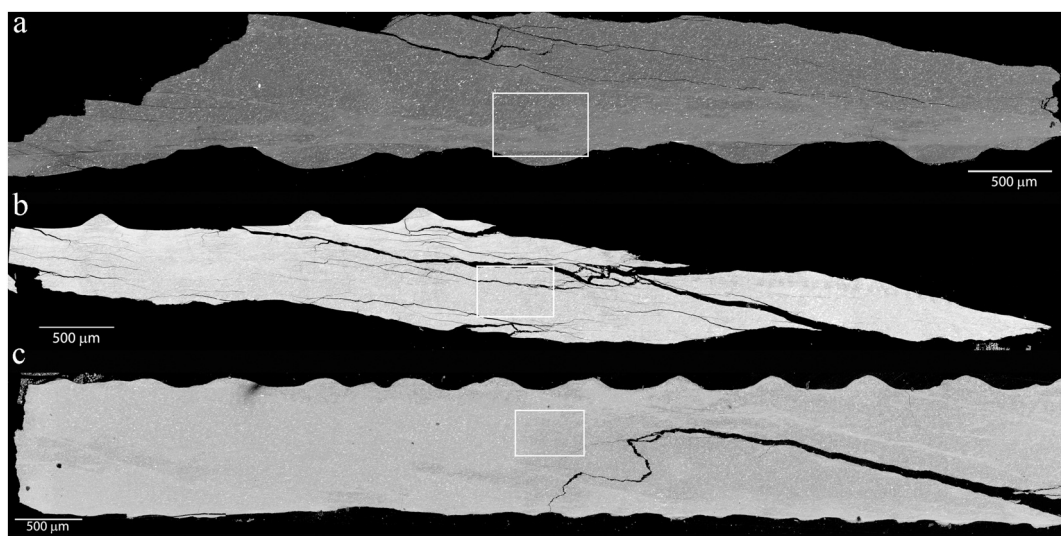
Fig. 12. Microstructures obtained in normal-stress-stepping experiments using the felsic sample at 1 \mu\text{m/s} and temperature of 600 (top), 650 (middle) and 700 ^{\circ}\text{C} (bottom). A faint foliation defined by aligned muscovite is present and denser zones are visible as lighter areas. These areas appear to increase in size with increasing temperature. Grey boxes indicate the locations of the close-ups, shown in Fig. 13. Shear stress is top-to-the-right in all cases.
