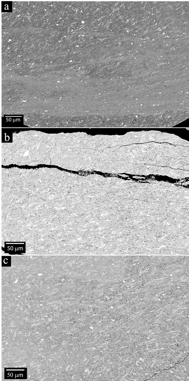
Fig. 13. Details of the microstructures of the felsic sample deformed at 1 \mu\text{m/s} and temperatures of 600 (a), 650 (b) and 700 °C (c). Shear sense is top-to-the-right in all cases.
