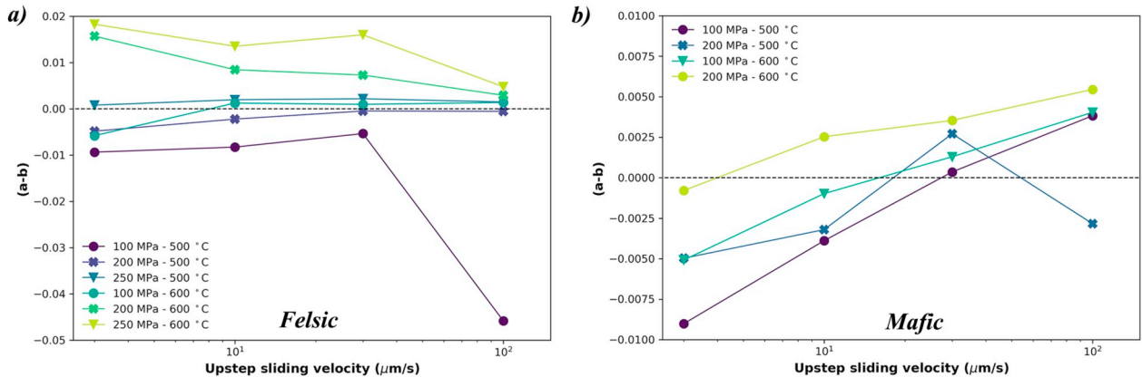
Fig. 7. a) Plots of (a-b) as a function of sliding velocity for experiments performed at effective normal stresses of 100, 200 and 250 MPa as well as 500 and 600 °C for the felsic sample.
