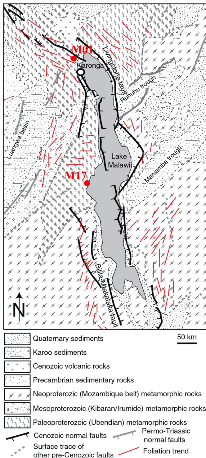
Fig. 1. Geologic map showing the sample locations (after Fagereng, 2013).
