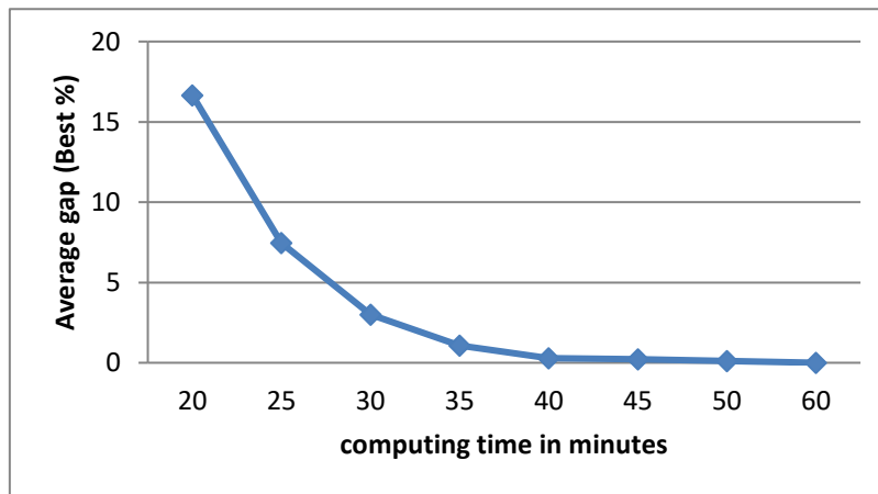
Fig.2. Average gap with respect to the best solution found after 60 minutes for large instances plotted against computing time
