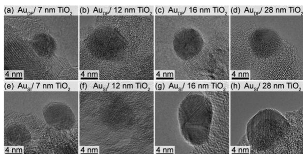
Figure 2. (a-d) HRTEM images of Au NPs deposited on TiO 2 with different crystallite sizes by DP method. (e-h) HRTEM images of Au NPs deposited on TiO 2 with different crystallite sizes by SI method.
