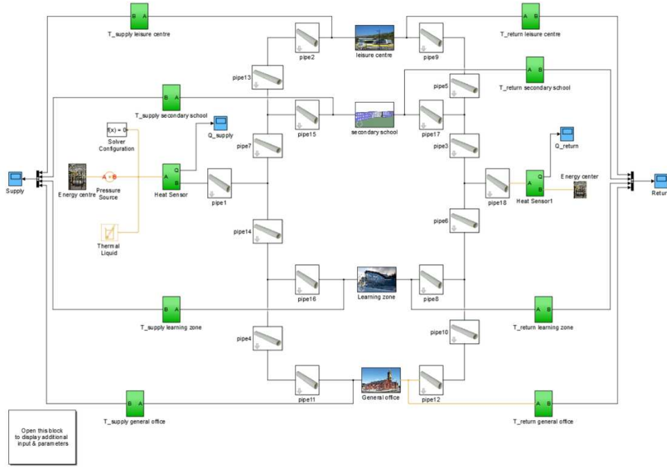
Fig. 7 The developed Simulink model for the distribution network
