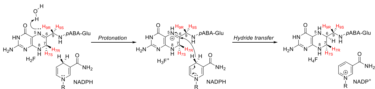
Figure 1. Reduction of 7,8-dihydrofolate (H 2 F) to 5,6,7,8-tetrahydrofolate (H 4 F) catalyzed by dihydrofolate reductase (DHFR). Hydrogens located at the β positions of the C6 of H 2 F are highlighted. p ABA-Glu = p -aminobenzoyl-L-glutamate.
