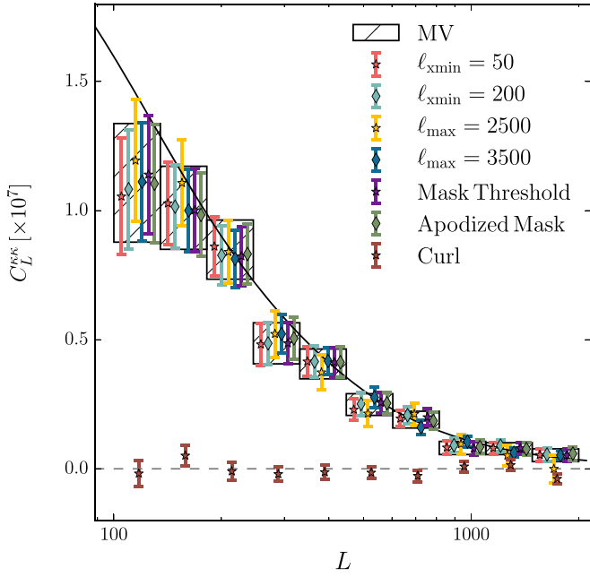
Figure 6. Results of the power spectrum consistency tests and curl null test. The figure shows C_L^{ns} bandpowers from different analysis choices and the curl test bandpowers. The MV bandpowers and error bars from the baseline analysis are plotted as boxes. The bandpowers calculated with different analysis choices are consistent with the baseline MV bandpowers. The bandpowers from the curl null test are consistent with zero.
