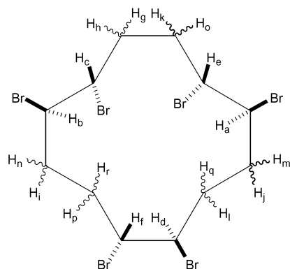
Fig. 7 Labeled structure of HBCD-2 (for explanation of the subscript letters, see experimental section).
