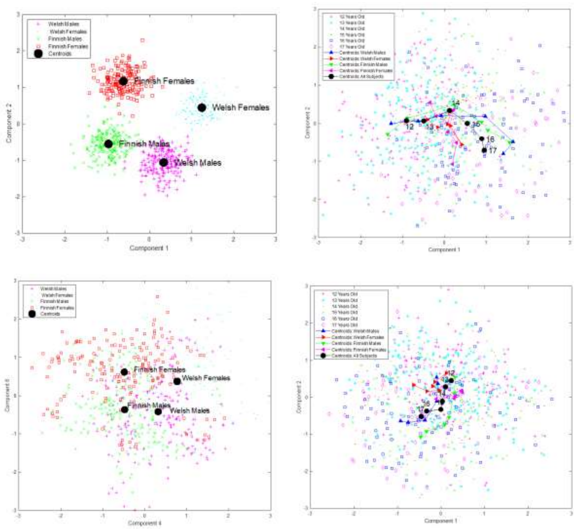
Figure 9: Standardised component scores via: top left, mPCA, level 1, components 1 and 2; top right, mPCA, level 3, components 1 and 2; bottom left, single-level PCA, components 4 and 3; bottom right, single-level PCA, components 2 and 1.
