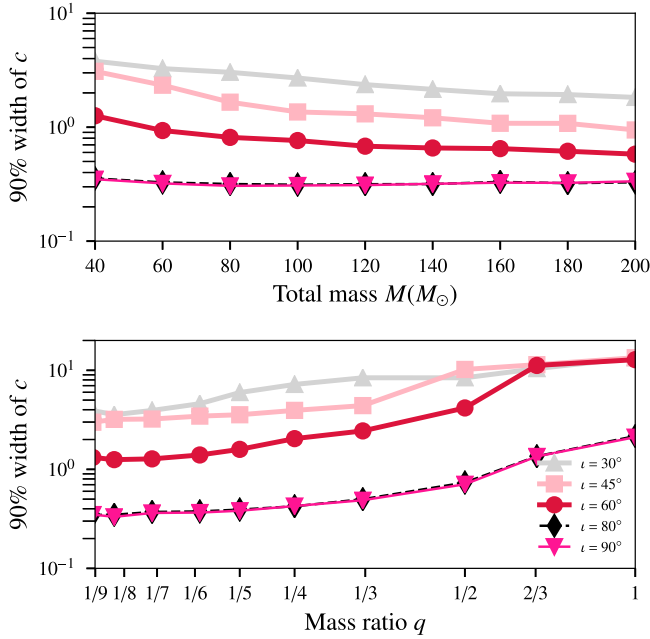
FIG. 7. The width of 90% credible regions of the posteriors of c for binaries with different total mass M (upper panel), mass ratio q (lower panel), and inclination angle \iota (legends). All binaries considered in the upper panel have a mass ratio q = 1/9 . Binaries considered in the lower panel have total mass of 40 M_{\odot} . All the simulated observations produce a network SNR of 25 in Advanced LIGO-Virgo network.
