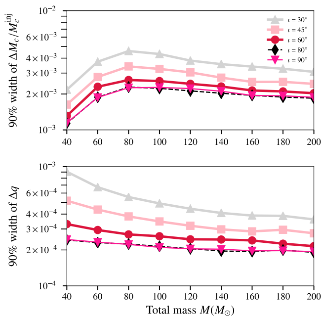
FIG. 3. The figure shows the width of the 90% credible regions of the deviation parameters \Delta M_c and \Delta q for binaries with different total mass (horizontal axis) and inclination angles \iota (legends). All binaries have an asymmetric mass ratio q = 1/9 .
