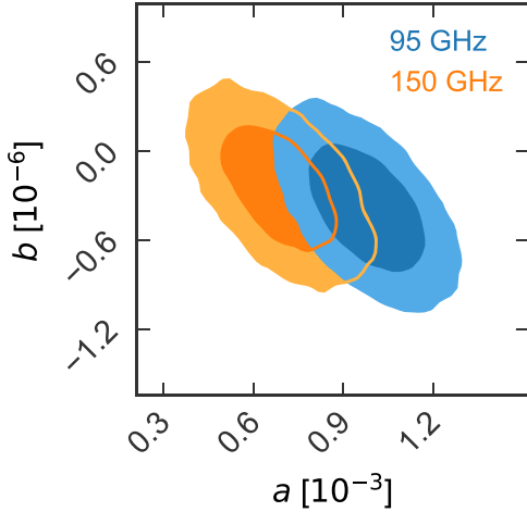
Figure 4. We find no evidence that the polarization fraction depends on the flux of the source at either 95 or 150 GHz. Here, we show the 1\sigma and 2\sigma contours from fitting the measured \langle p^2 \rangle values to a linear function of flux, \langle p^2 \rangle = a + b \times S , over the flux range S \in [6, 1500] mJy. The slope is consistent with zero at both frequencies. The shape of the degeneracy between the offset and slope can be understood by the fact the polarization fraction is well measured for bright sources, but increasingly uncertain towards lower fluxes. The errors at 95 GHz are larger due to higher map noise levels (see Section 2.2).
