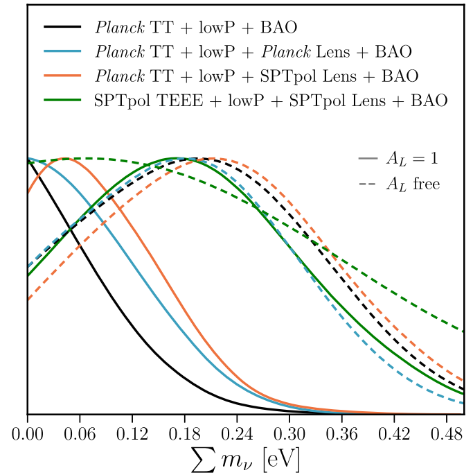
Figure 7. Constraints on the sum of the neutrino masses \sum m_\nu , when Planck primary CMB and BAO information is exploited (black line) and when either SPTPOL lensing (orange line) or Planck lensing (cyan line) is included in the cosmological analysis. If we replace the Planck primary CMB with the SPTPOL TEEE measurement from Henning et al. (2018) and include SPTPOL lensing and BAO, we obtain the green curve. Dashed lines show instead the results when we marginalize over the lensing information in the primary CMB (i.e., we let A_L free to vary).
