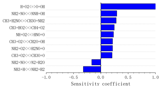
Fig. 18 Normalized sensitivity analysis on OH for 90%NH 3 /10%CH 4 fuel blend at ER=0.5, p=2atm, T=1550K.
