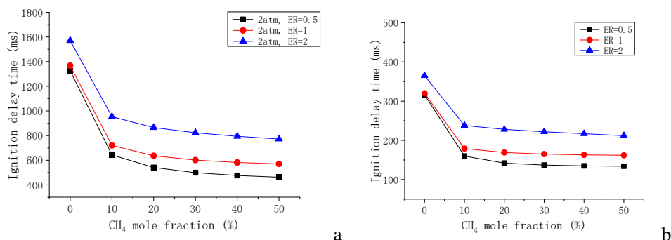
Fig. 11 Ignition delay time as a function of CH 4 mole fraction in NH 3 /CH 4 fuel blends at T=1550K (a) 2atm (b) 10atm
