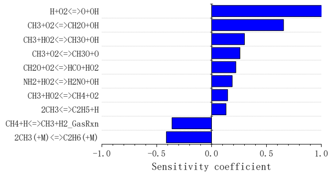
Fig. 14 Normalized sensitivity analysis on OH for 60%NH 3 /40%CH 4 fuel blend at ER=2, p=2atm, T=1550K.
