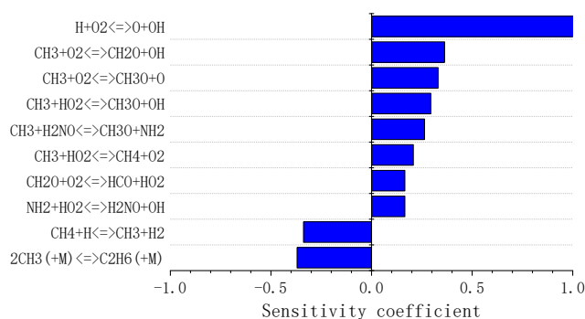
Fig. 12 Normalized sensitivity analysis on OH for 60%NH 3 /40%CH 4 fuel blend at ER=0.5, p=2atm, T=1550K.
