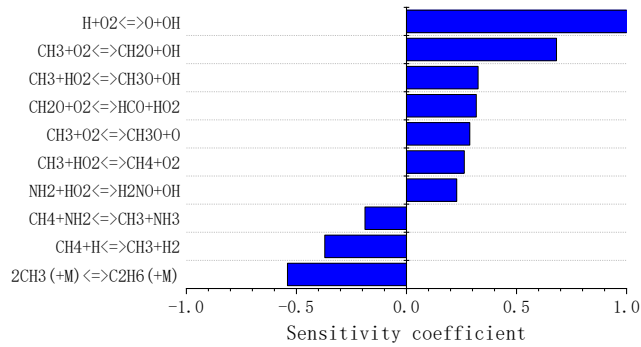
Fig. 16 Normalized sensitivity analysis on OH for 60%NH 3 /40%CH 4 fuel blend at ER=0.5, p=10atm, T=1550K.
