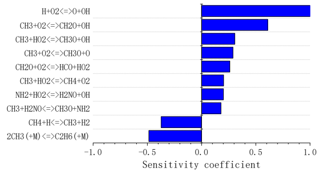
Fig. 15 Normalized sensitivity analysis on OH for 60%NH 3 /40%CH 4 fuel blend at ER=0.5, p=5atm, T=1550K.
