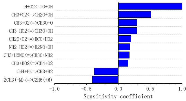
Fig. 13 Normalized sensitivity analysis on OH for 60%NH 3 /40%CH 4 fuel blend at ER=1, p=2atm, T=1550K.
