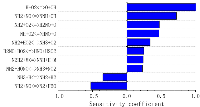
Fig. 17 Normalized sensitivity analysis on OH for pure NH 3 fuel at ER=0.5, p=2atm, T=1550K.
