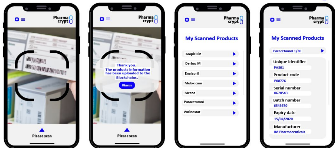
Figure 2: Proposed “Pharmacrypt” Application Tool User Interface.
