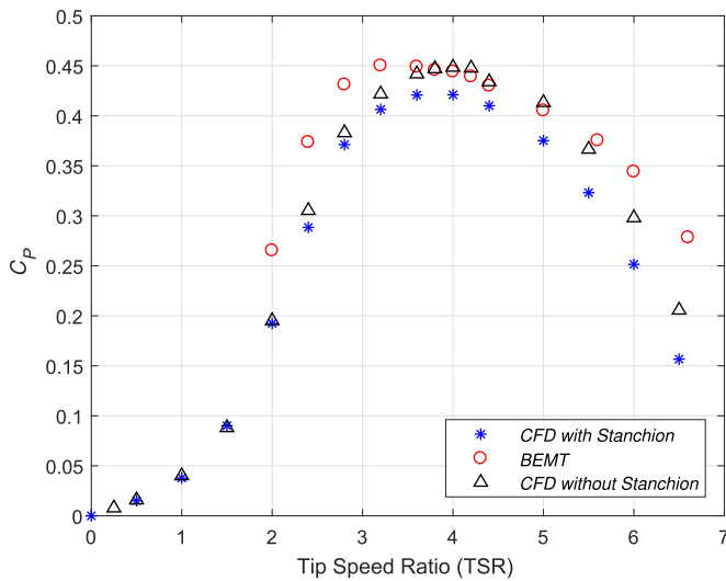
Fig. 4. Comparison of the C_p between CFD and BEMT.
