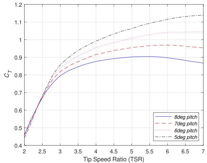
Fig. 3. Comparison of the BEMT C_T predictions for pitch angles of 5–8°.
