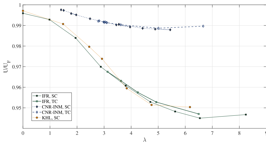
Fig. 9. The blockage ratio of constrained flow to open channel flow velocity, U/U_F , against \lambda values for the three differing test facilities.
