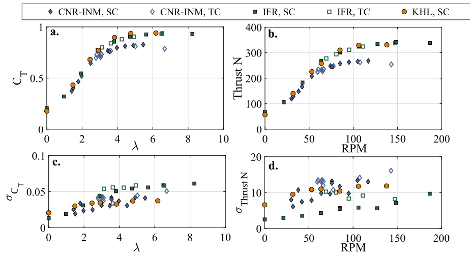
Fig. 12. Blockage corrected thrust curves obtained whilst testing at both CNR-INM and IFREMER. a) Shows Non-Dimensional thrust coefficient against \lambda . b) Shows thrust against RPM. c) Shows the standard deviation in non-dimensional thrust coefficient against \lambda . d) Shows the standard deviation in thrust against RPM.
