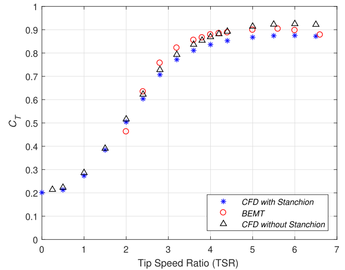
Fig. 5. Comparison of the C_T between CFD and BEMT.
