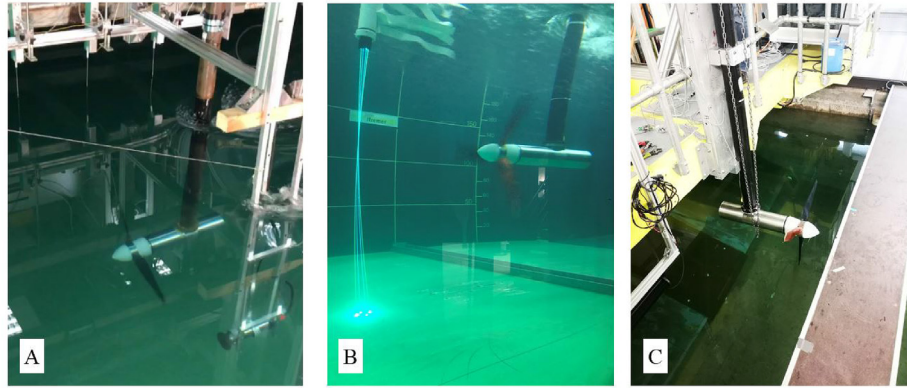
Fig. 8. The test setups at the various testing facilities, A) CNR-INM, B) IFREMER and C) KHL.
