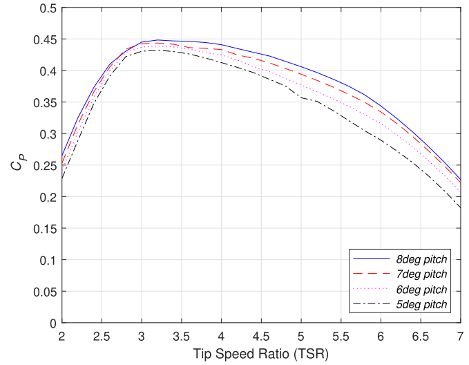
Fig. 2. Comparison of the BEMT C_p predictions for pitch angles of 5–8°.
