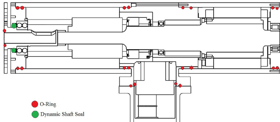
Fig. 7. Overview of the sealing arrangements for the 1/20th Scale HATT.
