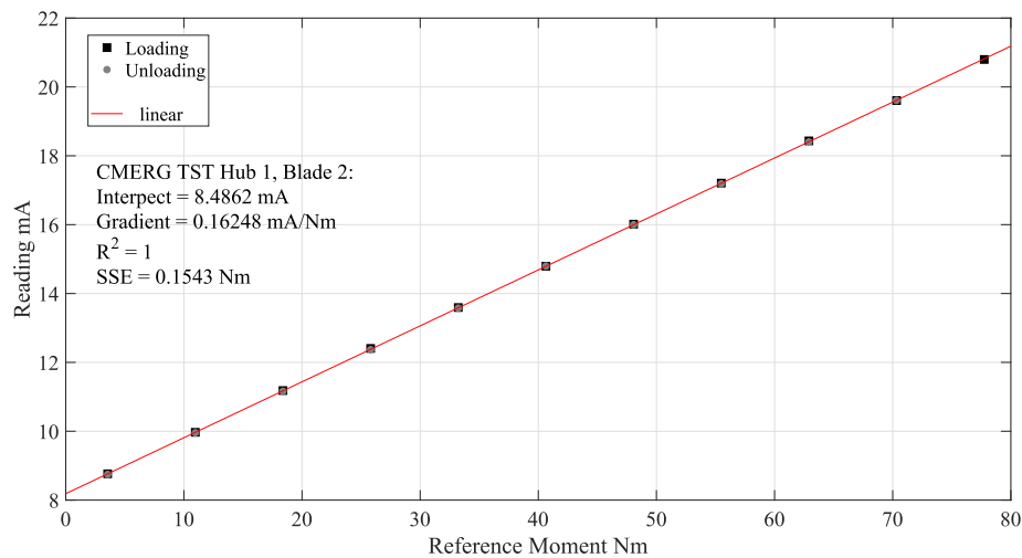
Fig. B20. The calibration results for the flapwise blade root bending moment transducer for blade 2, hub 1.
