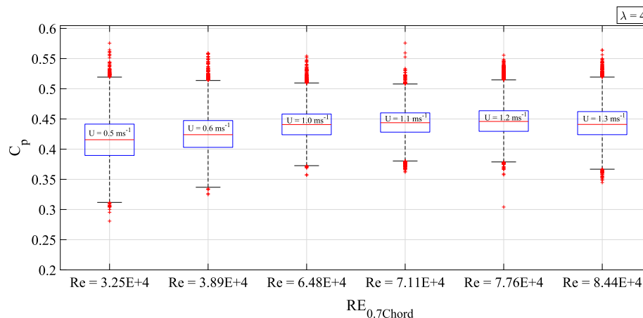
Fig. A19. Comparison of C_p values observed for tests under taken at differing fluid velocities. The C_p values are plotted against chord length based Reynold's Number for a fixed \lambda -value of \lambda = 4 .
