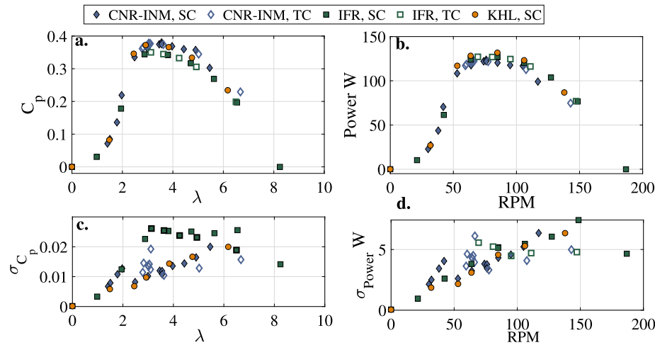
Fig. 10. Blockage corrected power curves obtained whilst testing at CNR-INM, IFREMER and KHL. a) Shows Non-Dimensional power coefficient against \lambda . b) Shows Power against RPM. c) Shows the standard deviation in non-dimensional power coefficient against \lambda . d) Shows the standard deviation of power against RPM.
