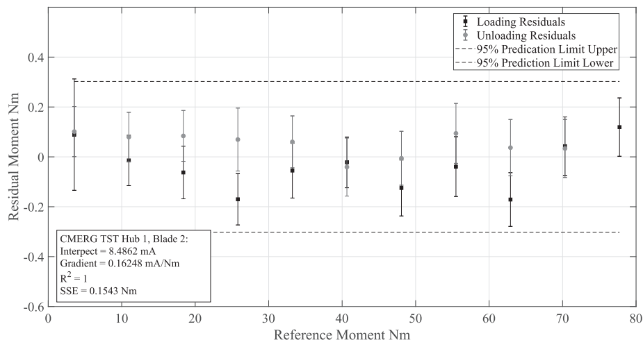
Fig. B21. Fitted residuals for calibration results for the flapwise blade root bending moment transducer for blade 2, hub 1.
