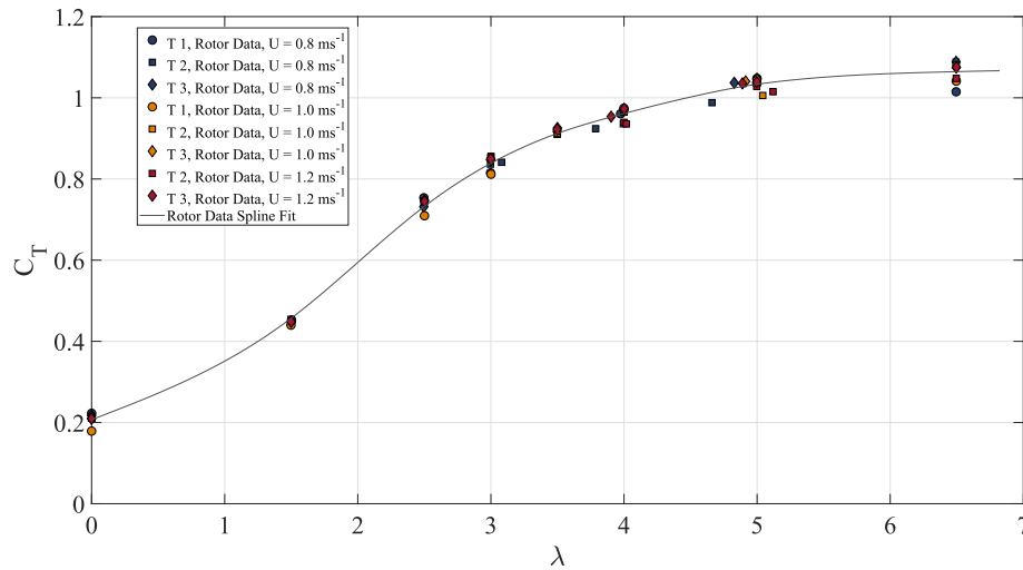
Fig. 16. Characteristic thrust curves obtained whilst testing at KHL for each of the three turbines.
