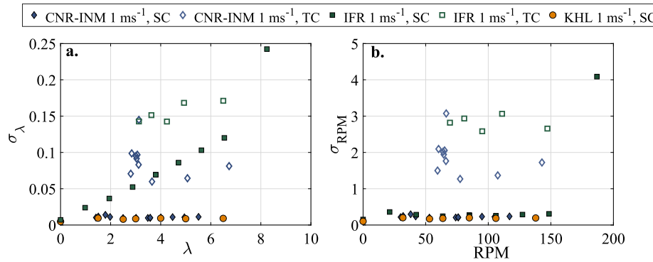
Fig. 13. Figure showing the standard deviation of \lambda values against \lambda (left) and the standard deviation of RPM against RPM (right).
