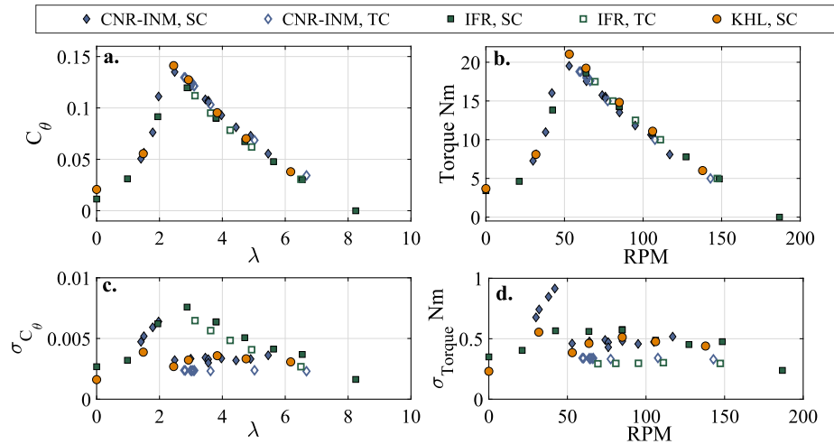
Fig. 11. Blockage Corrected torque curves obtained whilst testing at CNR-INM, IFREMER and KHL. a) Shows Non-Dimensional torque coefficient against \lambda . b) Shows torque against RPM. c) Shows the standard deviation in non-dimensional torque coefficient against \lambda . d) Shows the standard deviation in torque against RPM.
