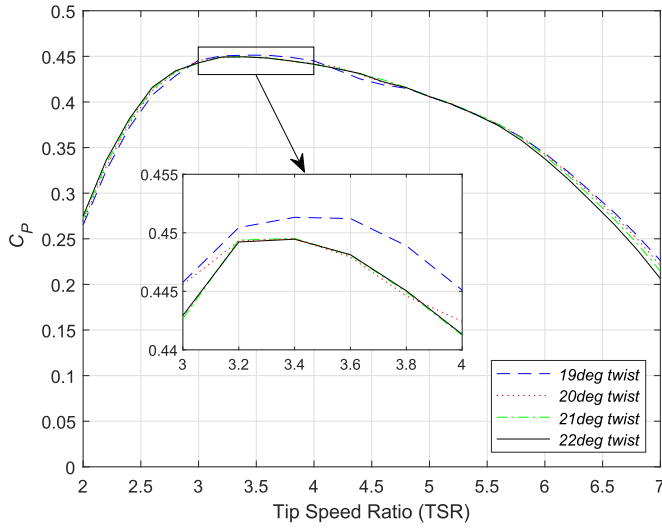
Fig. 1. Comparison of the BEMT C_p predictions for twist distributions between 19 and 22°.
