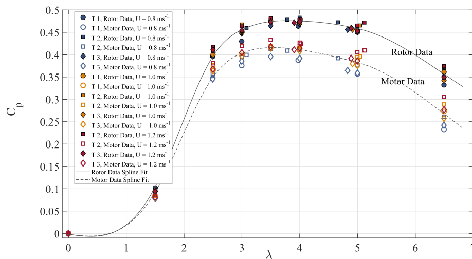
Fig. 14. Characteristic power curves obtained whilst testing at KHL for each of the three turbines, the figures show both the power curves obtained considering rotor transducer measurements and motor power measurements.
