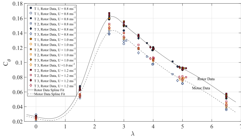
Fig. 15. Characteristic torque curves obtained whilst testing at KHL for each of the three turbines, the figures show both the power curves obtained considering rotor transducer measurements and motor power measurements.
