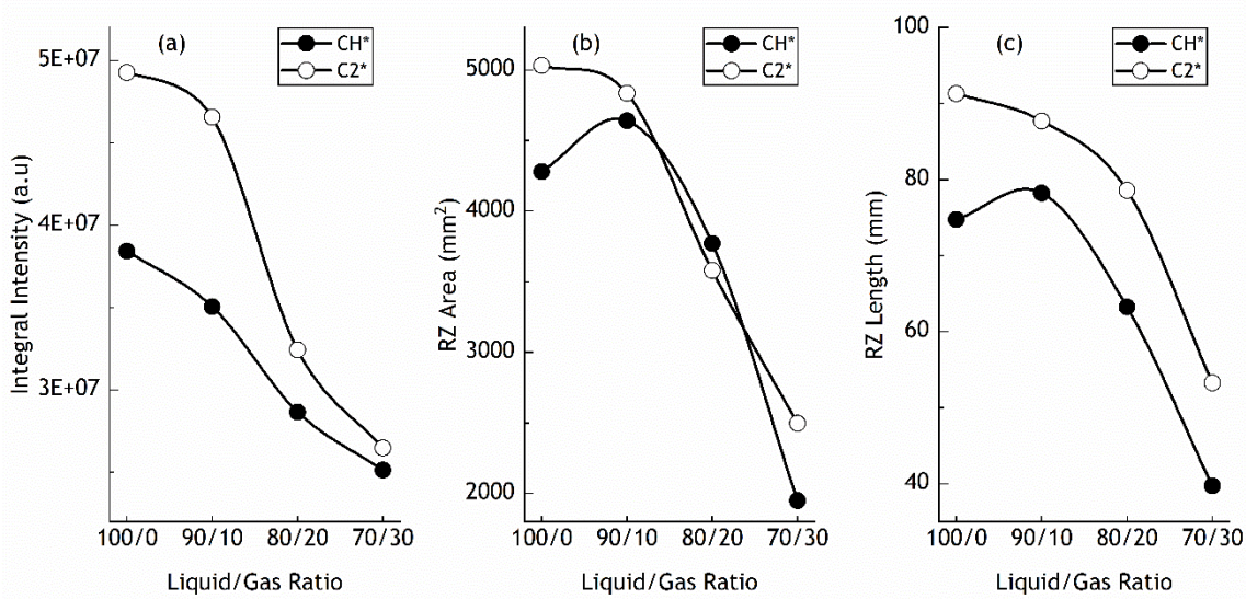
Fig. 5. Reaction zone properties: (a) species integral intensity, (b) reaction zone (RZ) area and (c) reaction zone length of 15 kW biodiesel/methane flames at \phi_{\text{global}} = 0.7
