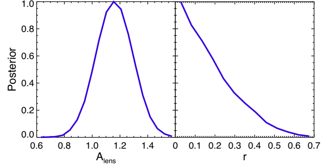
FIG. 3. The measured B -mode power spectrum is consistent with the Planck best-fit \Lambda\text{CDM} model. On the left, we show the posterior probability for A_{\text{lens}} ( A_{\text{lens}} rescales the predicted B -modes due to lensing), finding it consistent with unity. In the right panel, we show that the posterior probability for the tensor-to-scalar ratio r peaks at zero.
