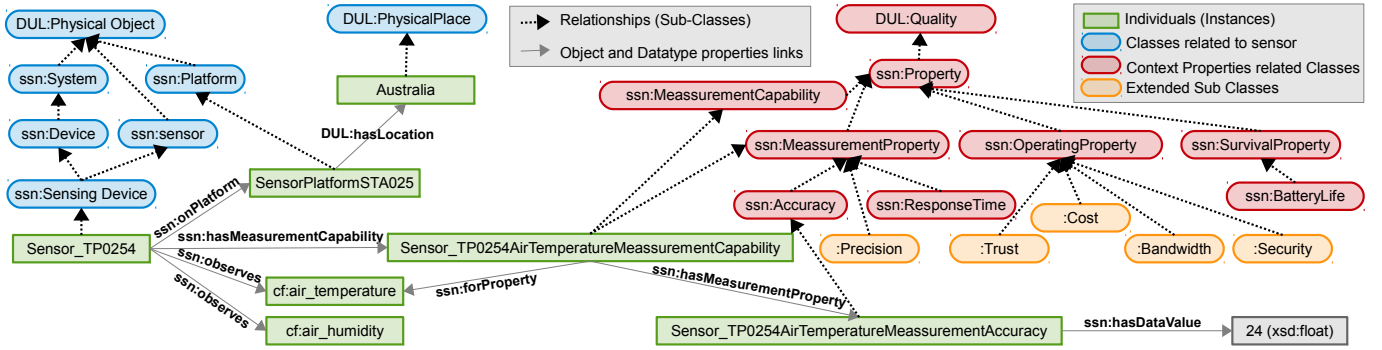
Fig. 3: Data model used in CASSARAM. In SSN ontology, sensors are not constrained to physical sensing devices; rather a sensor is anything that can estimate or calculate the value of a phenomenon, so a device or computational process or combination could play the role of a sensor. A sensing device is a device that implements sensing [5]. Sensing device is also a sub class of sensor . By following above definition, our focus is on sensors. CF (Climate and Forecast) ontology is a domain specific external ontology. DOLCE+DnS Ultralite (DUL) ontology provides a set of upper level concepts that can be the basis for easier interoperability among many middle and lower level ontologies. More details are provided in [5].
