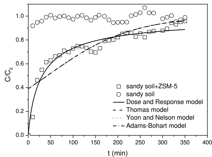
57 Figure 9 The experimental and predicted breakthrough curves for the adsorption of 58 MTBE on sand and sand-ZSM-5 mixture at an inlet MTBE concentration of 300 \text{ mg}\cdot\text{L}^{-1}
