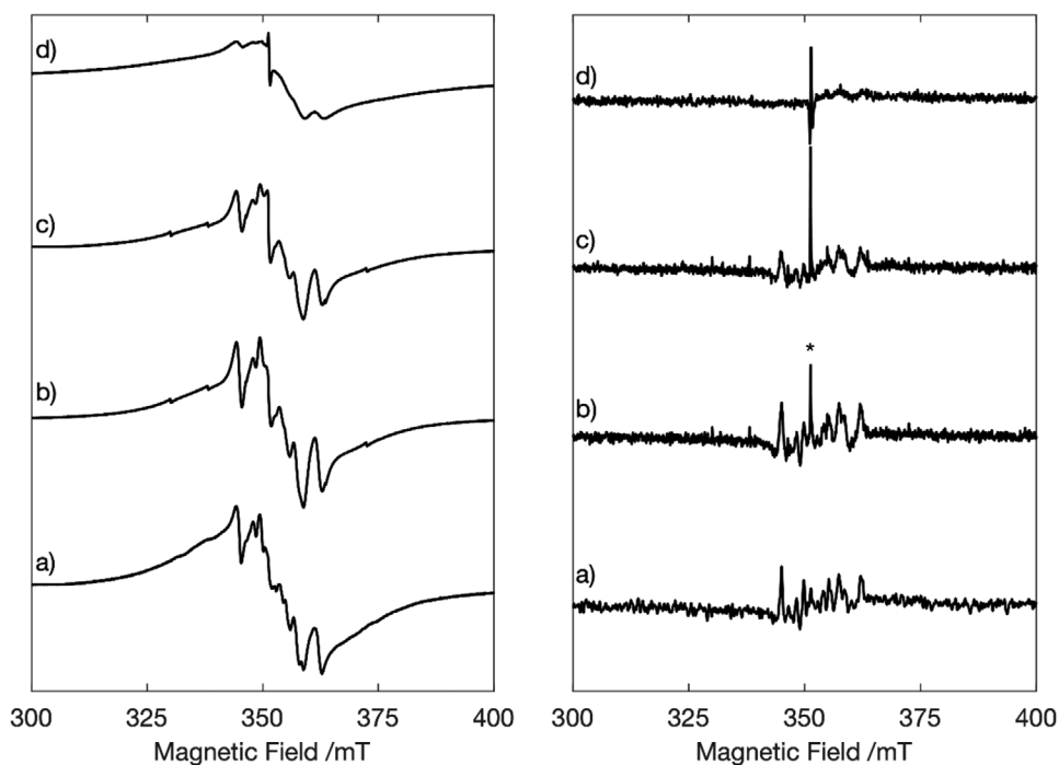
Figure 4. CW X-band (9 GHz) EPR spectra (120 K) of a) the native CaSEu_Na sample, after b) one (CaSEu_Na_C1), c) two (CaSEu_Na_C2), and d) three (CaSEu_Na_C3) consecutive cryo-milling treatments. Left: Standard first derivative measurements; Right: second derivative measurements indicating onset of V_S' center signal, labeled by an asterisk.
