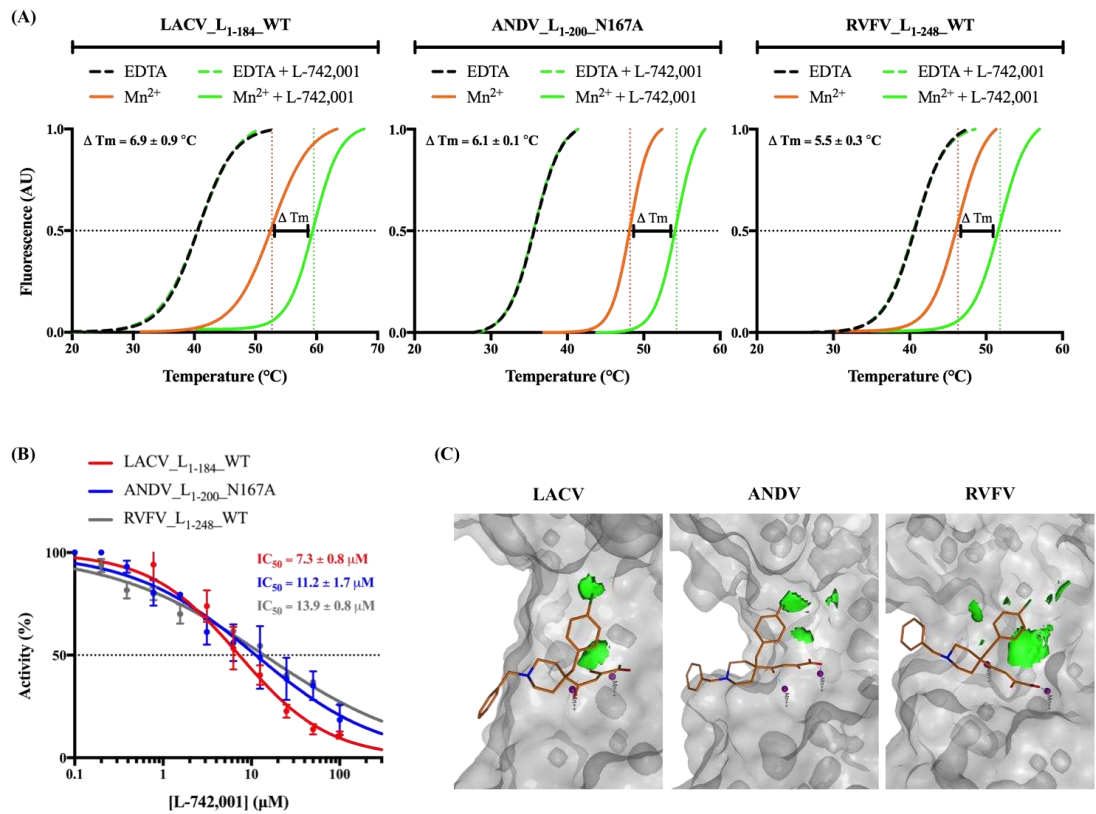
Fig. 2. L-742,001 inhibitory molecular interactions with Bunyavirales Cap-ENDO's. (A) Thermal stability of LACV_L1-184_WT (left panel), ANDV_L1-200_N167A (middle panel) and RVFV_L1-248_WT (right panel) in the presence of 10 mM EDTA (black dashed line), 10 mM EDTA plus 25 μM L-742,001 (green dashed line), 10 mM MnCl 2 (orange solid line) and 10 mM MnCl 2 plus 25 μM L-742,001 (green solid line). The compound contribution to the stability of the proteins was determined by the difference in T m between the samples containing MnCl 2 in the presence and absence of L-742,001 ( \Delta T_m ). The lines depict the non-linear fits of the normalized fluorescence curves to the Boltzmann equation. (B) Dose-dependent inhibition of the nuclease activity of LACV_L1-184_WT (red), ANDV_L1-200_N167A (blue) and RVFV_L1-248_WT (grey) by L-742,001. The reactions were initiated with the addition of 1 μM of FRET-labeled ssRNA substrate to the pre-incubated mixtures of 0.25 μM of the respective enzymes with two-fold serial dilutions of L-742,001. The fluorescent
