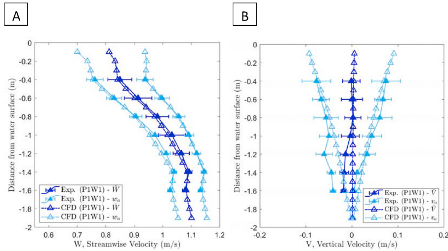
Fig. 15. For P1W1, the average and wave orbital A) streamwise and; B) vertical, CFD and experimental velocity results. Bars show \pm 1 standard deviation. [ \bar{W} or \bar{V} = average velocity, w_a or v_a = maximum and minimum wave orbital velocity component].
