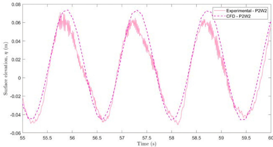
Fig. 20. The experimental and CFD surface elevation for the conditions given by P2W2.
