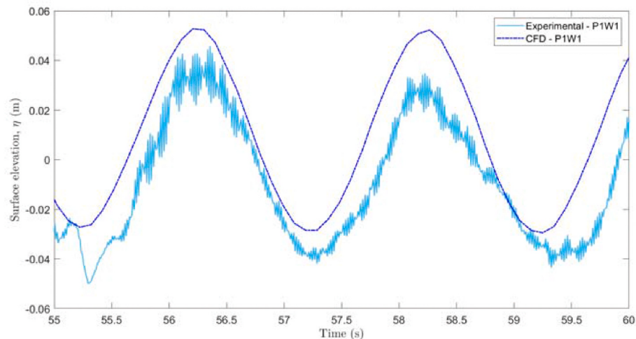
Fig. 19. The experimental and CFD surface elevation for the conditions given by P1W1.
