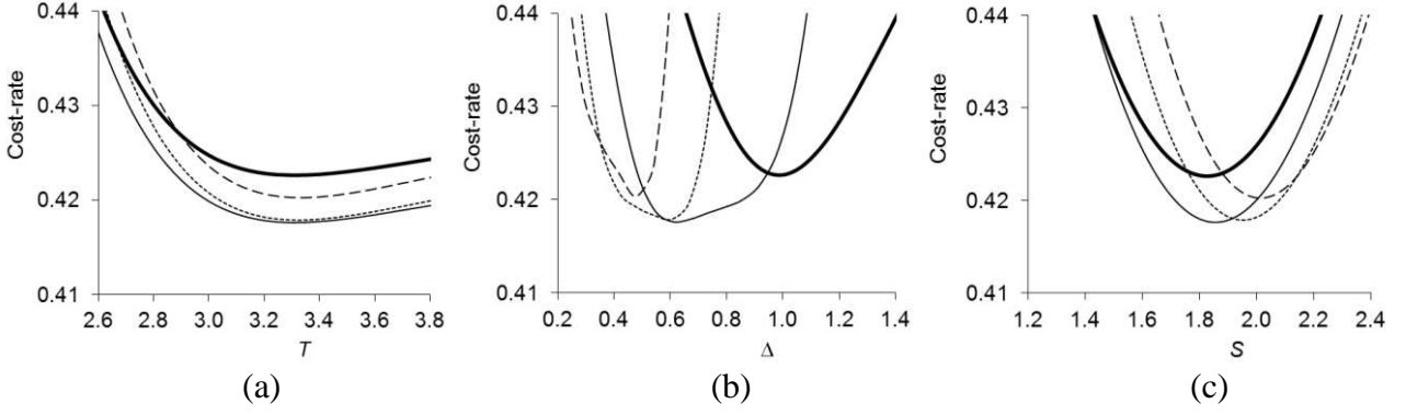
Figure 5. For policy 1, cost-rate versus (a) age at preventive replacement T , (b) interval between inspections \Delta , (c) threshold age for opportunity S , for K=1 (—), K=2 (— —), K=3 (-----); K=4 (- -); other decision variables held in turn at their respective optimum values; parameter values as case 1: \beta_1 = 2.5 , \eta_1 = 0.8 , \beta_2 = 5 , \eta_2 = 3.6 , p = 0.1 , \mu = 2 , \lambda = 1 , C_1 = 0.03 , C_O = 0.5 , C_F = 5 , C_R = 1 .
