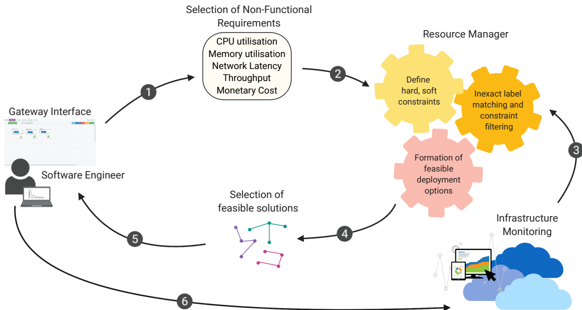
FIGURE 1 Decision-making process for continuous adaptation of AI-based microservices as part of a software engineering life-cycle, for cloud-native applications.
