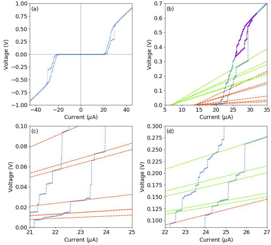
Figure 4: V(I) characteristic of the 6.7 \mu\text{m} wide BNCD microbridge switched by electromagnetic noise. (a) The full V(I) characteristic measured at 1.9 \text{ K} for the same sample as shown in Fig. 3 switched into the metastable resistive state near to I_R by an applied electromagnetic noise pulse during the upward current sweep. (b) Detail of the hysteresis region close to I_R . A repeatable hysteresis loop (purple) can be traced if the bias current is not returned to zero after switching. (c), (d) Details of individual current-voltage steps, showing converging linear slopes with selected fit lines for clarity. Red lines converge to I_0 = 13.78 \mu\text{A} ; green lines converge to I_1 = 6.89 \mu\text{A} .
