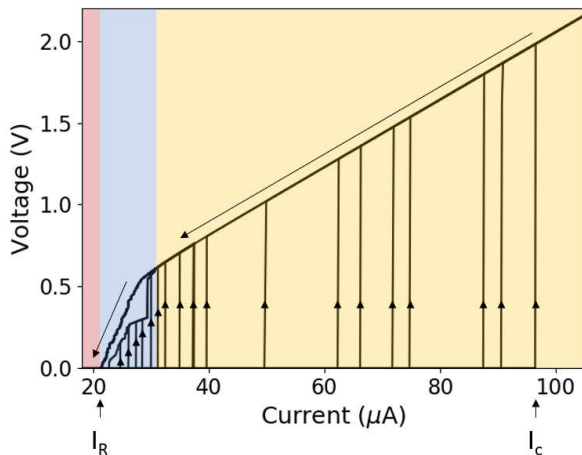
Figure 5: Controlled electromagnetic noise pulse induced switching of the 6.7 \mu\text{m} wide BNCD microbridge state. The bias current through the microbridge at 1.9K is repeatedly ramped above I_c and then back to below I_R . On each ramp the noise pulse is applied to coincide with a different value of bias current on the rising path. The plot is a composite of all ramps; the points at which the pulses were applied are shown by the vertical arrows on the graph. The colored regions are as described in the main text.
