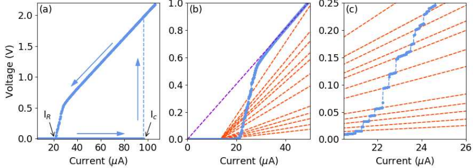
Figure 3: Current-biased V(I) characteristic for a 6.7 \mu\text{m} wide, 339 \text{ nm} thick BNCD microbridge at 1.9 \text{ K} . Only the positive current branch is shown for clarity. (a) I_c and I_R denote the critical current and retrapping current respectively. The arrows show the current direction around a hysteretic loop. (b) An expanded view of the falling current branch showing discrete voltage steps with subsequent linear slopes that converge to the same point I_0 = 13.78 \mu\text{A} on the current axis. (c) A detailed view of individual voltage steps, showing the converging linear slopes.
