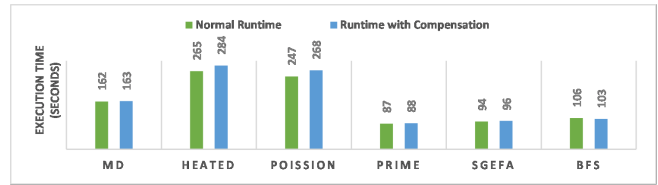
Figure 20: Effect of power capping with compensation on parallel workloads on ARM.
