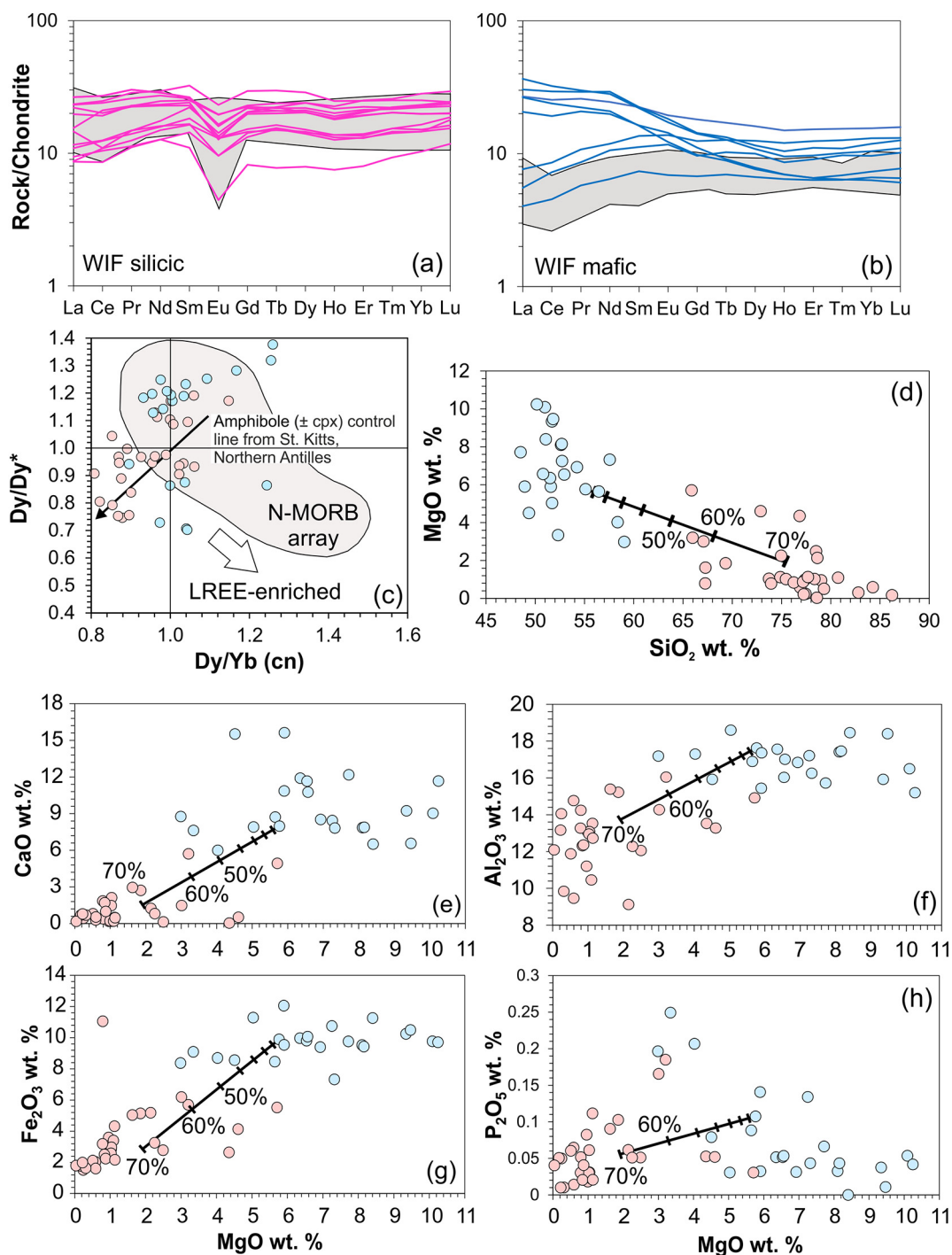
Fig. 8. (a and b) Chondrite-normalised REE diagrams showing raw data from this study and grey fields representing analyses from Jolly and Lidiak (2006). (c) Dy/Dy*–Dy/Yb cn diagram from Davidson et al. (2013) and (d–h) major element bivariate diagrams showing fractional crystallisation trends of a plagioclase (58%), clinopyroxene (10%), magnetite (12%), orthopyroxene (10%), amphibole (9.7%) and apatite (0.3%) mineral assemblage from a parental magma representing WIF sample SJ53. Tick marks on trends represent 10% increments. Virgin Island data in c–h are from this paper and Jolly and Lidiak (2006). Normalising values from McDonough and Sun (1995).
