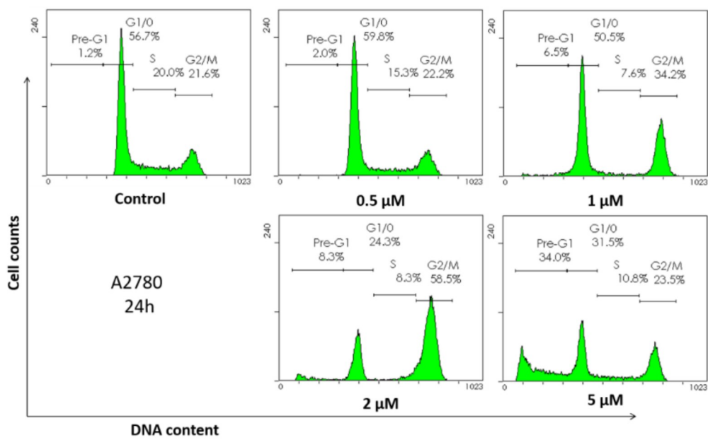
Fig. 7. Cell cycle effects of 30m . A2780 cells were treated with 30m for 24 h, followed by propidium iodide (PI) staining and analyzed by flow cytometry. Representative of three independent experiments is shown.
