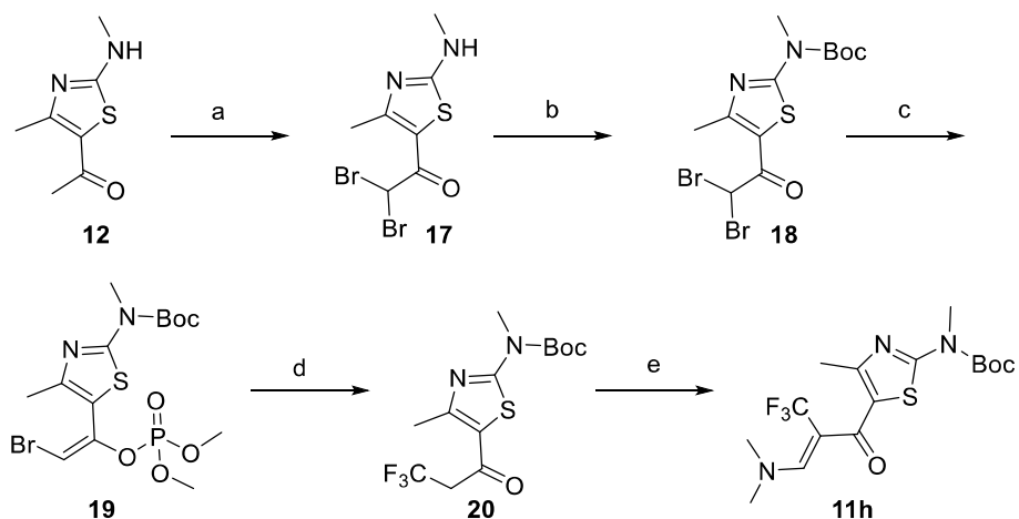
Scheme 3: Reagents and conditions: (a) Br 2 , 48% HBr solution, 60 °C, 3 h, 56 %; (b) Boc 2 O, DMAP, CH 2 Cl 2 , RT, 2 h; (c) trimethylphosphite, RT, 22 h; (d) FO 2 SCF 2 CO 2 CH 3 , CuI/DMF, 80 °C, overnight, 37 % over 3 steps; (e) DMA-DMA, Δ, 1 h, 64 %.
