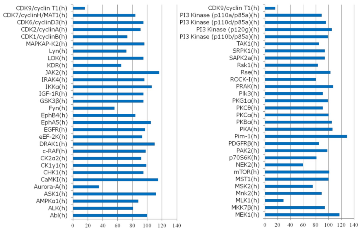
Fig. 4. Diversity kinase panel screening of 30m . The assay was carried out in duplicate. Percentage of remaining kinase activity is shown.
