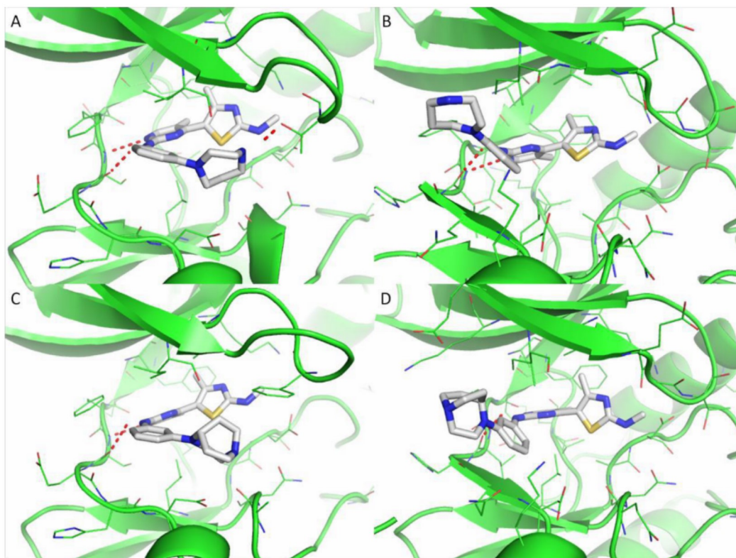
Fig. 3. Docking poses for complexes of CDK9 and CDK2 with compound 30k and 30m . (A): CDK9/ 30k ; (B): CDK2/ 30k ; (C): CDK9/ 30m ; (D): CDK2/ 30m . The kinase is presented in green in cartoon representation and selected residues are drawn in lines mode. Carbon atoms of 30k and 30m are grey and hydrogen bonds are denoted by red dashed lines.
