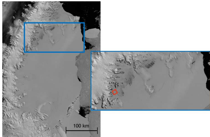
Figure 1. NASA MODIS imagery of the Larsen C Ice Shelf (Scambos et al., 2001). The image was captured on 7 January 2007 at 13:15. The presence of melt lakes is shown through the zoomed image of the northern part of Larsen C, where the red outlined area shows the location of the data used to produce Fig. 4.
