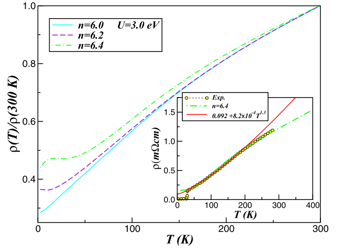
FIG. 5. T dependence of electrical resistivity (normalized at 300 K) for pure and electron-doped ThFeAsN, showing visible doping dependence below 100 K. Inset: theory-experiment comparison of resistivity versus temperature normalized to the experimental value at T_c = 30 K [11,12]. Notice the good agreement between theory, experiment, and the fitting curve from 215 K down to T_c .
