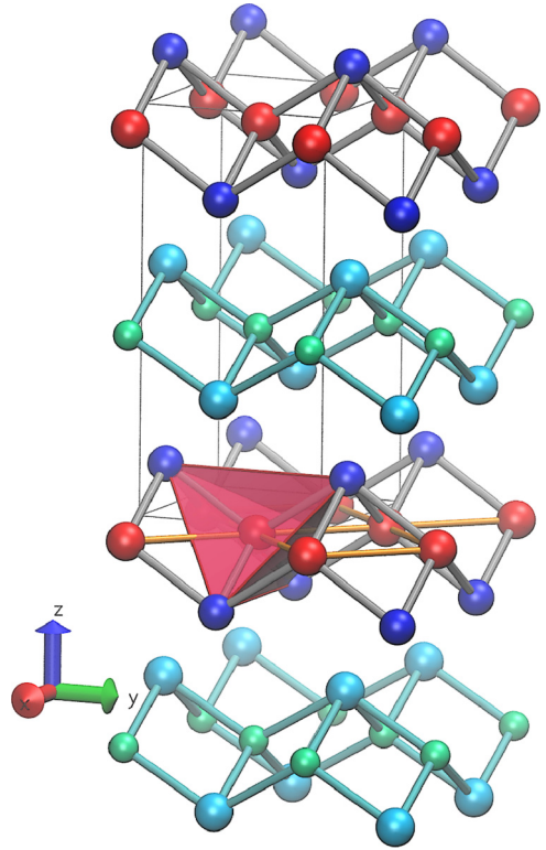
FIG. 1. Crystal structure of tetragonal ThFeAsN superconductor (Fe red, As blue, Th light-blue, N green). The tetragonal coordination of Fe by As is represented as a red tetrahedron. Within a single layer, the square planar arrangement of Fe atoms is shown (orange connections). The tetragonal unit cell is drawn in gray.
