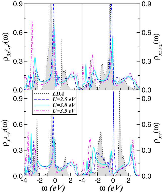
FIG. 2. LDA and LDA + DMFT orbital resolved density-of-states (DOS) of a tetragonal ThFeAsN superconductor, showing spectral weight redistribution over large energy scales with increasing onsite Coulomb interaction U . While all orbitals are metallic at U = 2.5 eV, orbital-selective localization within the xy orbital sets in for U = 3.0 eV. Particular interesting features to be seen are the peak-dip-hump within the 3z^2 - r^2, xy, yz, x^2 - y^2 orbitals and the local moment (lower Hubbard band) formation in the 3z^2 - r^2 orbital at U = 3.5 eV.
