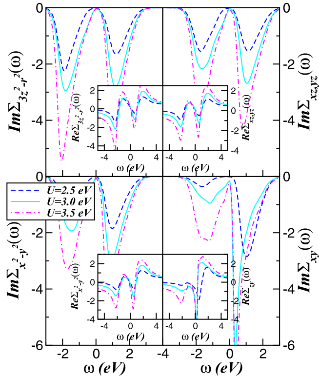
FIG. 3. Orbital-resolved self-energies imaginary (main panels) and real (insets) parts of ThFeAsN parent compound, showing their evolution with increasing U for fixed J_H = 0.7 eV. Particular features seen are the particle-hole asymmetry and the almost perfect Fermi liquid ( \omega^2 ) behavior of Im\Sigma_a(\omega) ( a = 3z^2 - r^2, xz, yz, x^2 - y^2 ), suggesting the coexistence of itinerant electrons and nearly Mott localized electronic states with xy orbital character in the unconventional electronic fluid of ThFeAsN. Also interesting is the frequency dependence of the self-energy real parts, showing orbital dependent electron correlation effects.
