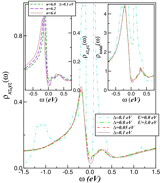
FIG. 6. xz , yz and total spectral functions in the single gap s -wave superconducting state [13] of a bulk ThFeAsN crystal, showing their evolution with changing the pair-field \Delta and fixed n = 6.4 (main and right inset panels), and by enhancing the electron band filling with fixed \Delta = 0.1 eV (left inset panel). Notice the particle-hole asymmetry and the nearly similar correlated spectral functions at low energies. Also noteworthy are the Bogoliubov quasiparticles obtained in the U = 0.0 eV limit, which are strongly reshaped due to dynamical spectral weight transfer induced by multiorbital electron interactions at energies above the s -wave superconducting gap.
