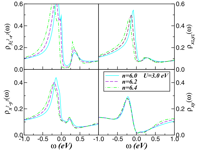
FIG. 4. Low energy view of orbital resolved spectral functions of pure and electron-doped ThFeAsN. Notice the robustness of the xy pseudogapped electronic state and the emergence of a Kondo insulating state with 3z^2 - r^2 orbital character upon increasing the total electron band filling of the Fe-3d shell.
