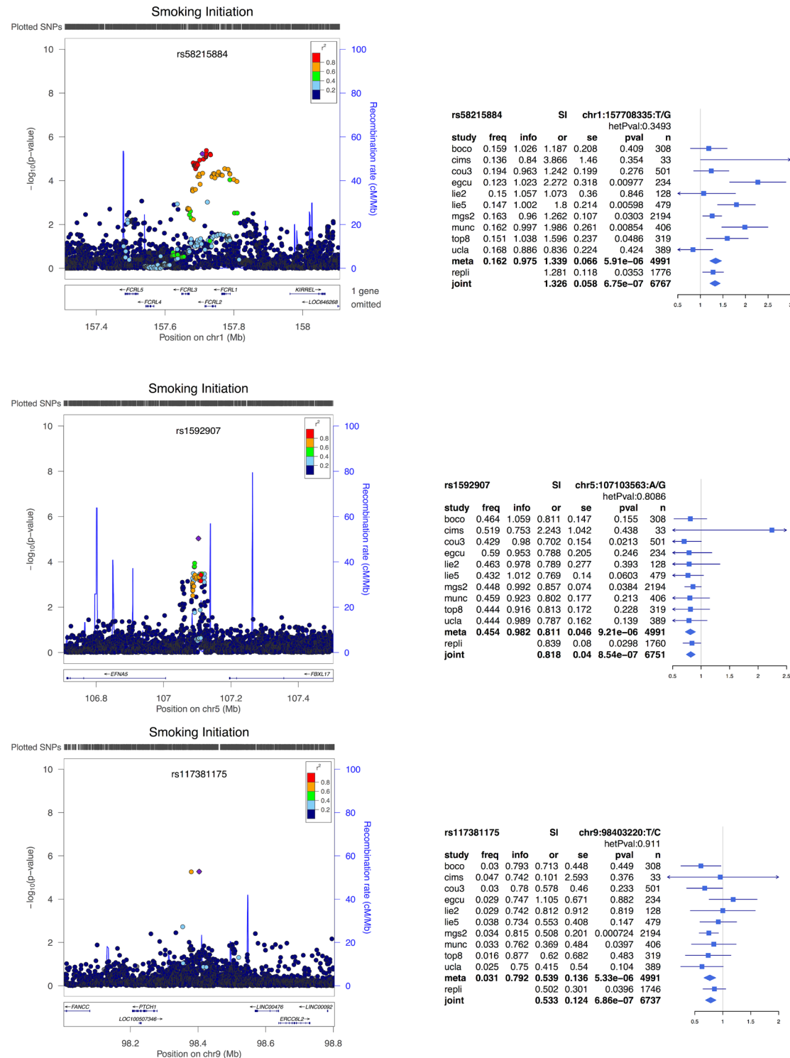
Figure S7. Regional association and forest plots for SI associations. ( left ) Regional association plot created using LocusZoom (22). LD of each SNP with the “index” SNP, displayed as a large purple diamond, is indicated by its color. ( right ) Study abbreviation “repli” is the replication sample; all other study indicators are as given above; HetP is the P -value for Cochran’s test of heterogeneity.
