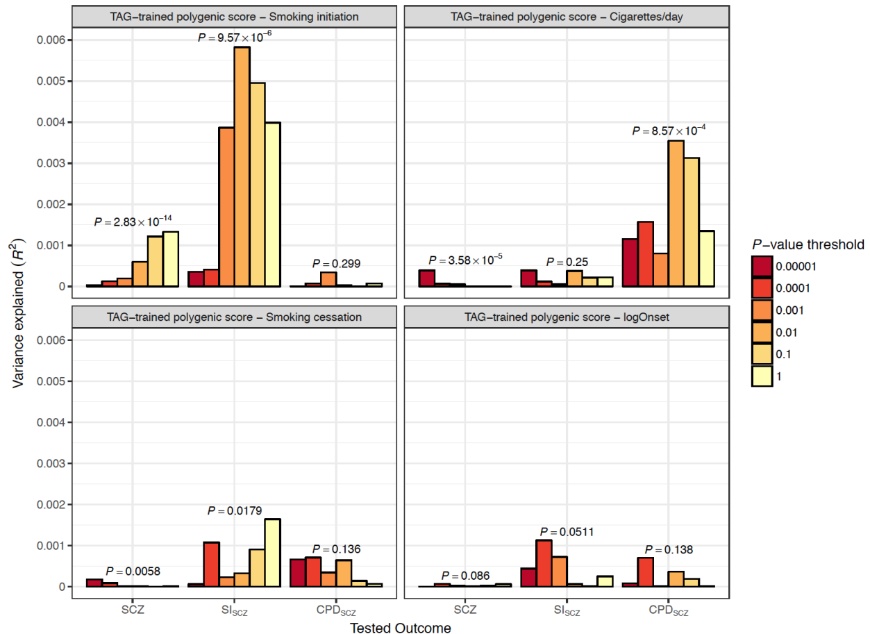
Figure 1. Association of TAG-based polygenic scores with schizophrenia risk and smoking behaviors. For polygenic scores based on analyses of smoking behaviors described by TAG, the variance explained for selected outcomes in PGC-schizophrenia is shown on the y-axis, in terms of Nagelkerke's pseudo- R^2 (schizophrenia and smoking initiation) or R^2 (cigarettes-smoked-per-day); scores based on varying SNP P -value inclusion thresholds are displayed as colored bars. logOnset is log-transformed age-of-onset (see Methods).
