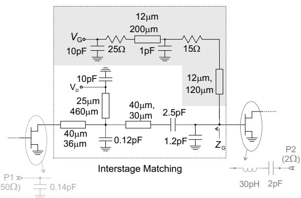
Fig. 4. Interstage matching network with microstrip lines' width and length. Equivalent input and output circuits of the final and driver device, extracted from cold-FET simulations, are also reported.
