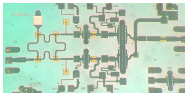
Fig. 5. DPA microscope picture ( 2.81 \times 1.35 \text{ mm}^2 ).
