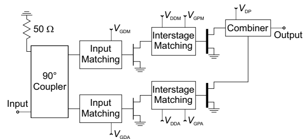
Fig. 1. DPA block diagram.
